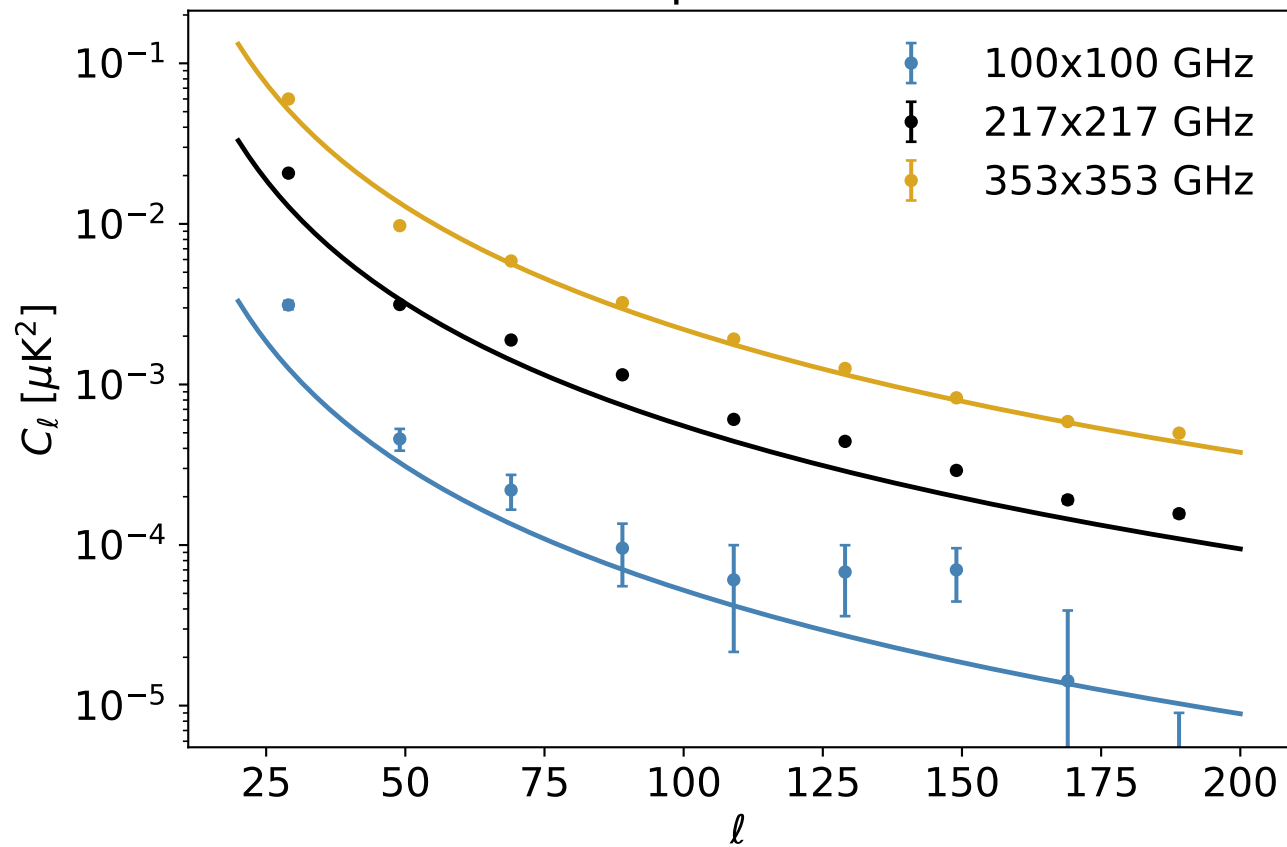
Auto-spectra — EE
