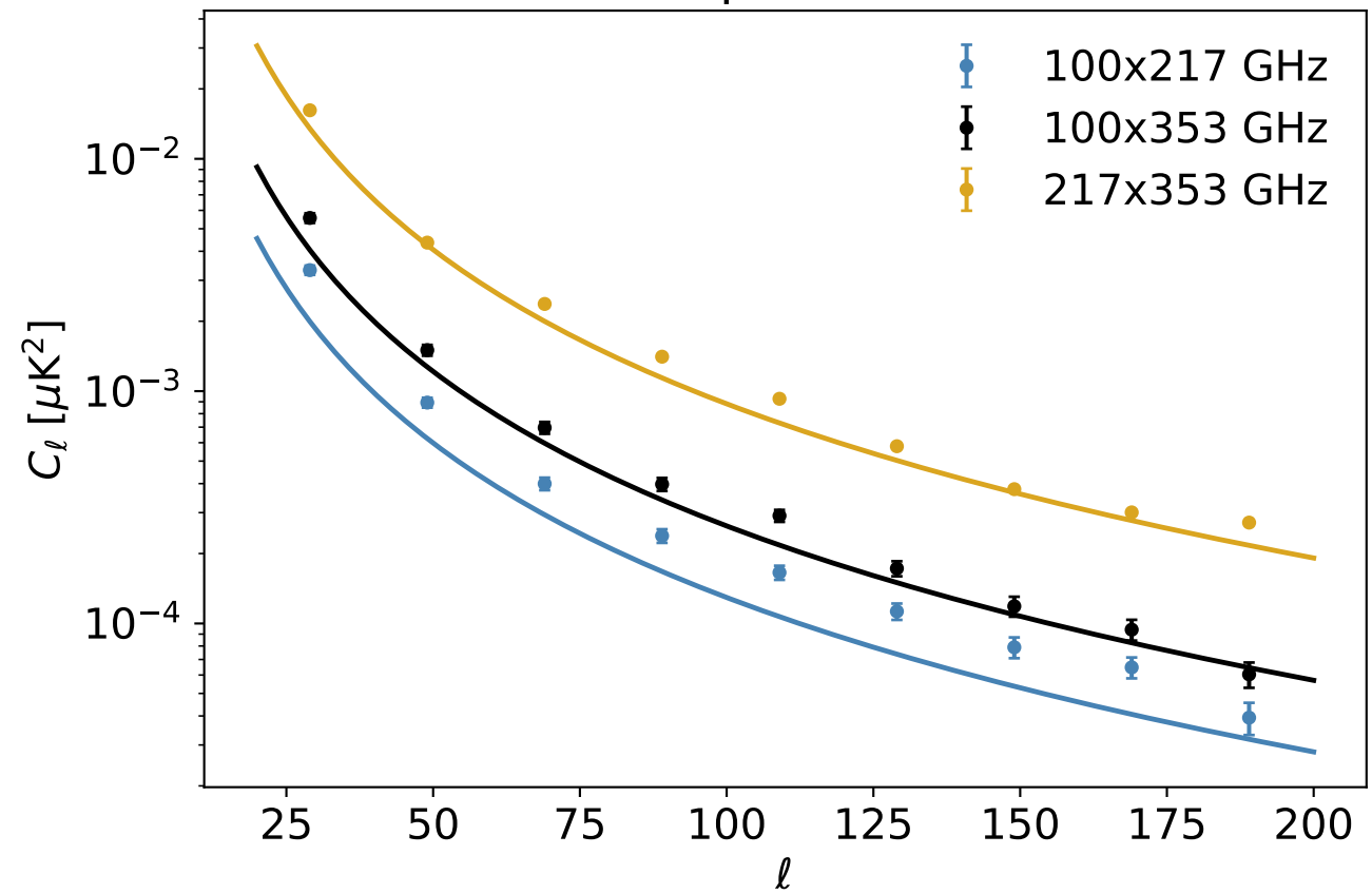
Cross-spectra — BB
