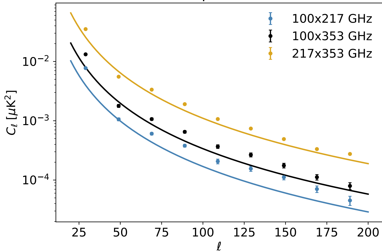
Cross-spectra — EE
