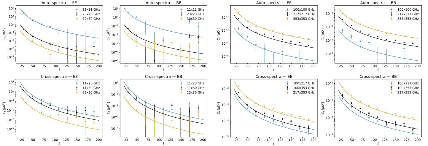
Figure 5: Best-fit global power-law models for synchrotron and thermal dust emission using cross-only spectra for the fit, overlaid on the measured EE and BB frequency power spectra, for the |b| > 10^\circ Galactic mask.
