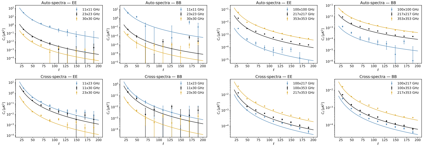
Figure 2: Best-fit global power-law models for synchrotron and thermal dust emission overlaid on the measured EE and BB frequency power spectra, for the |b| > 10^\circ Galactic mask.
