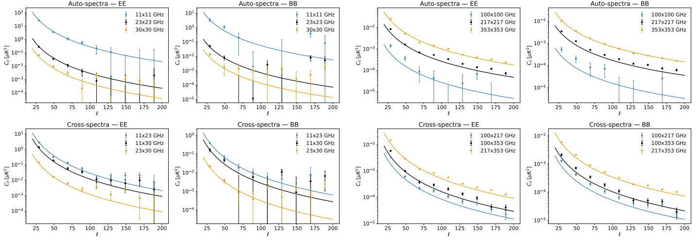
Figure 6: Same as Figure 5 but for the |b| > 20^\circ Galactic mask.
