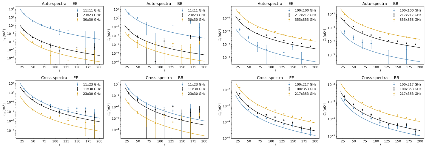
Figure 7: Same as Figure 5 but for the |b| > 20^\circ Galactic mask.
