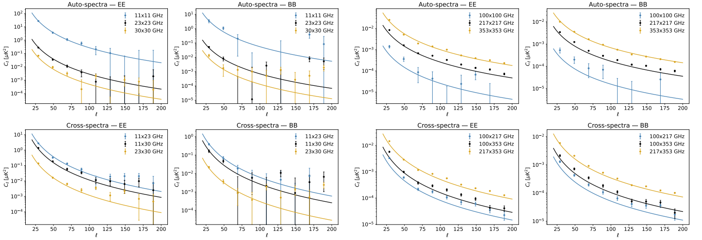
Figure 4: Best-fit global power-law models for synchrotron and thermal dust emission overlaid on the measured EE and BB frequency power spectra, for the |b| > 20^\circ Galactic mask.
