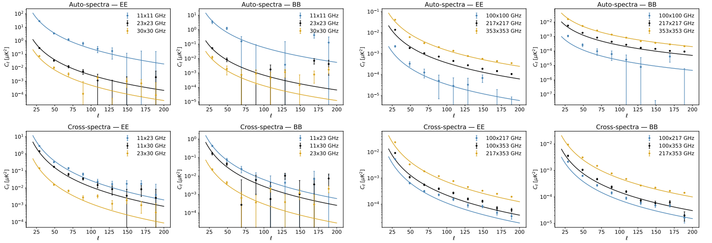
Figure 3: Best-fit global power-law models for synchrotron and thermal dust emission overlaid on the measured EE and BB frequency power spectra, for the |b| > 15^\circ Galactic mask.
