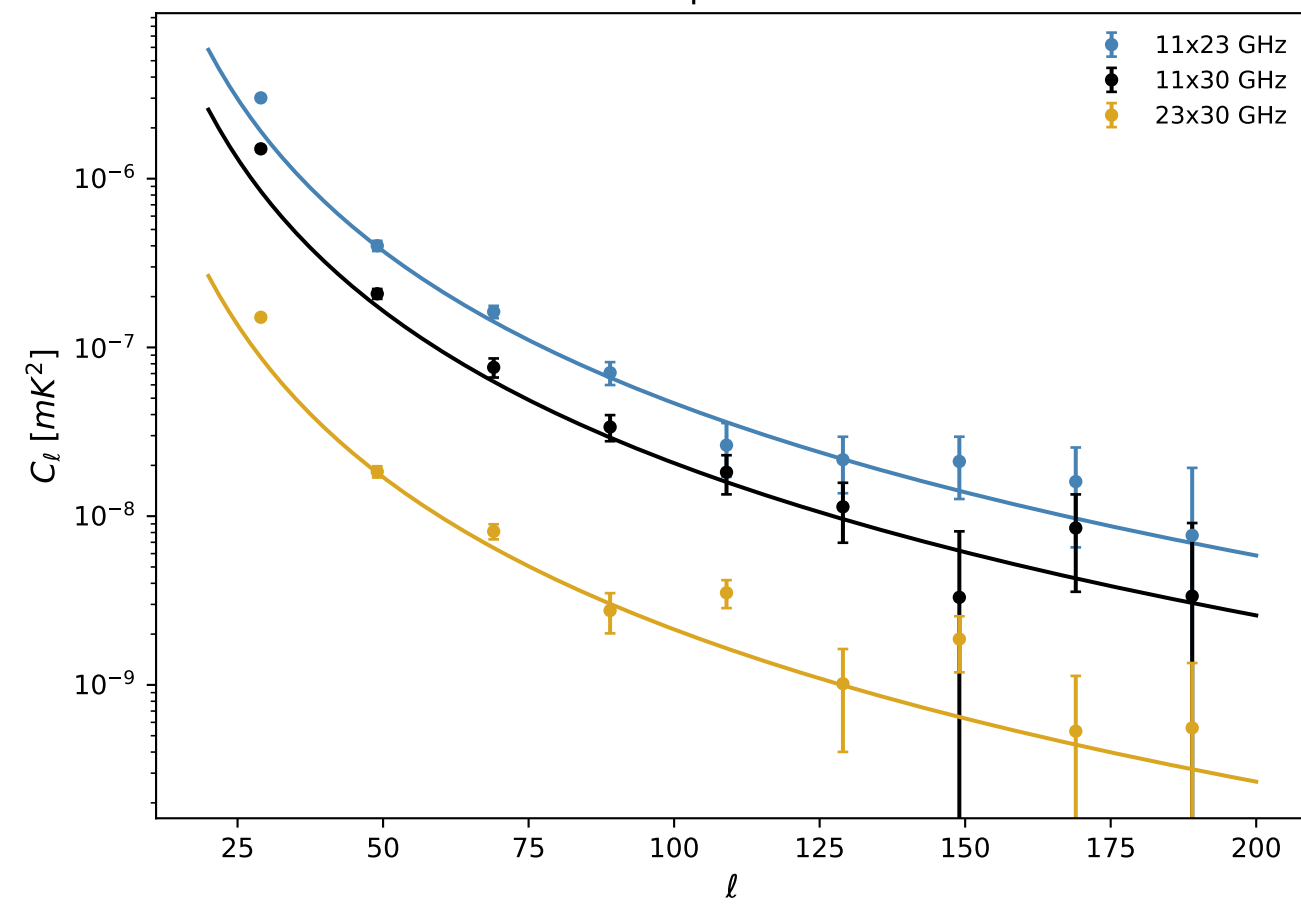
Cross-spectra — EE
