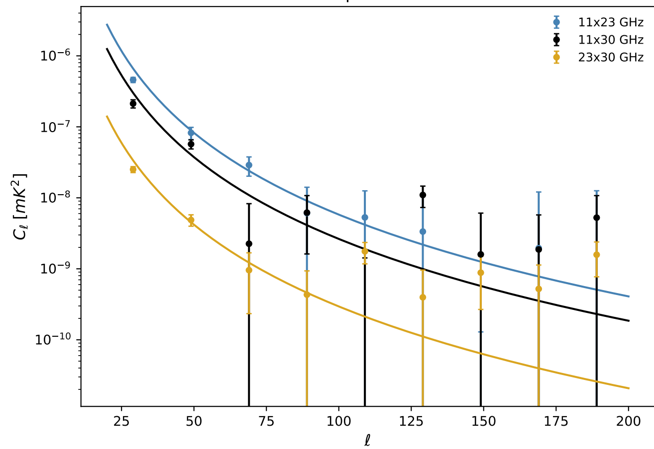
Cross-spectra — BB
