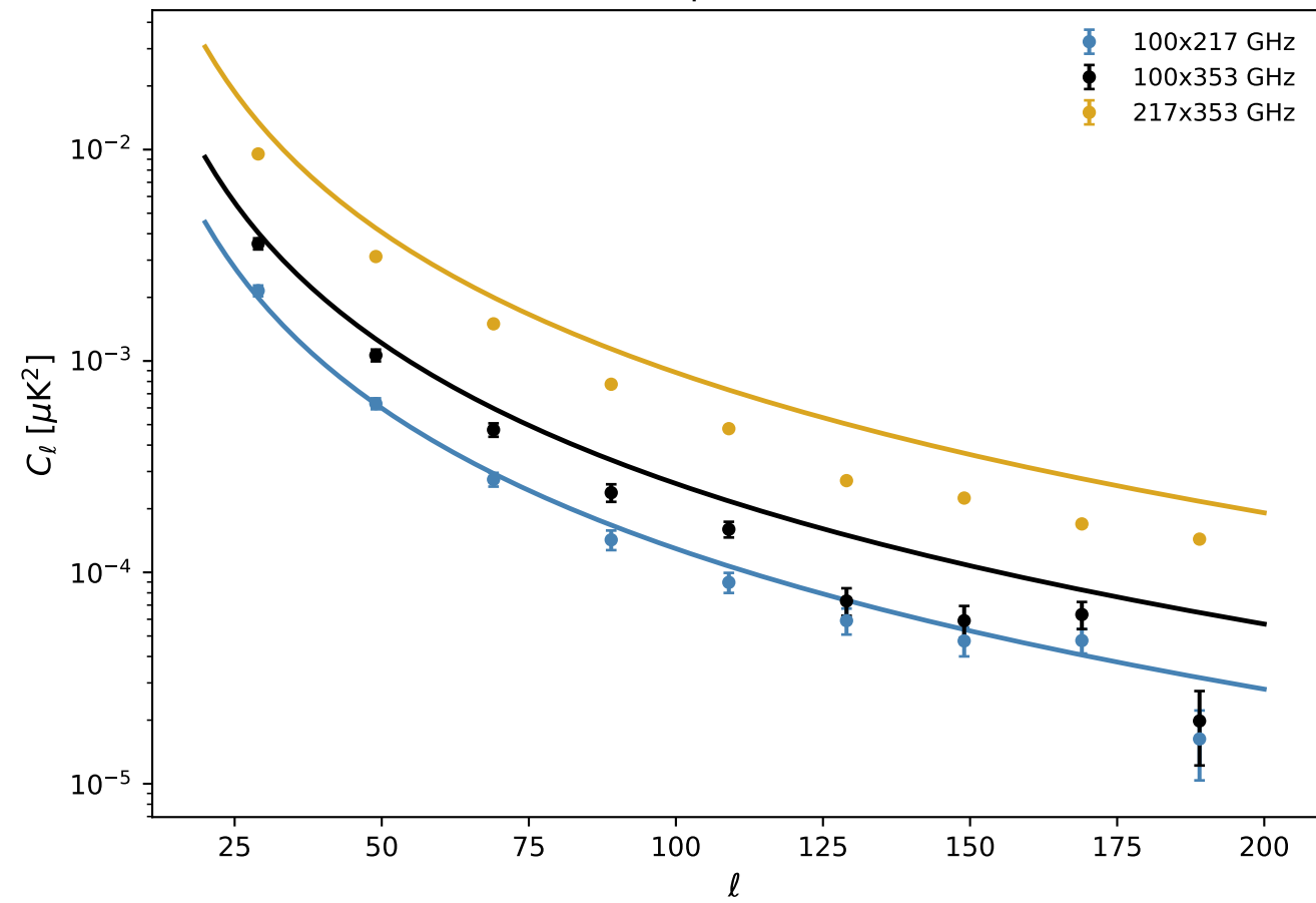
Cross-spectra — BB
