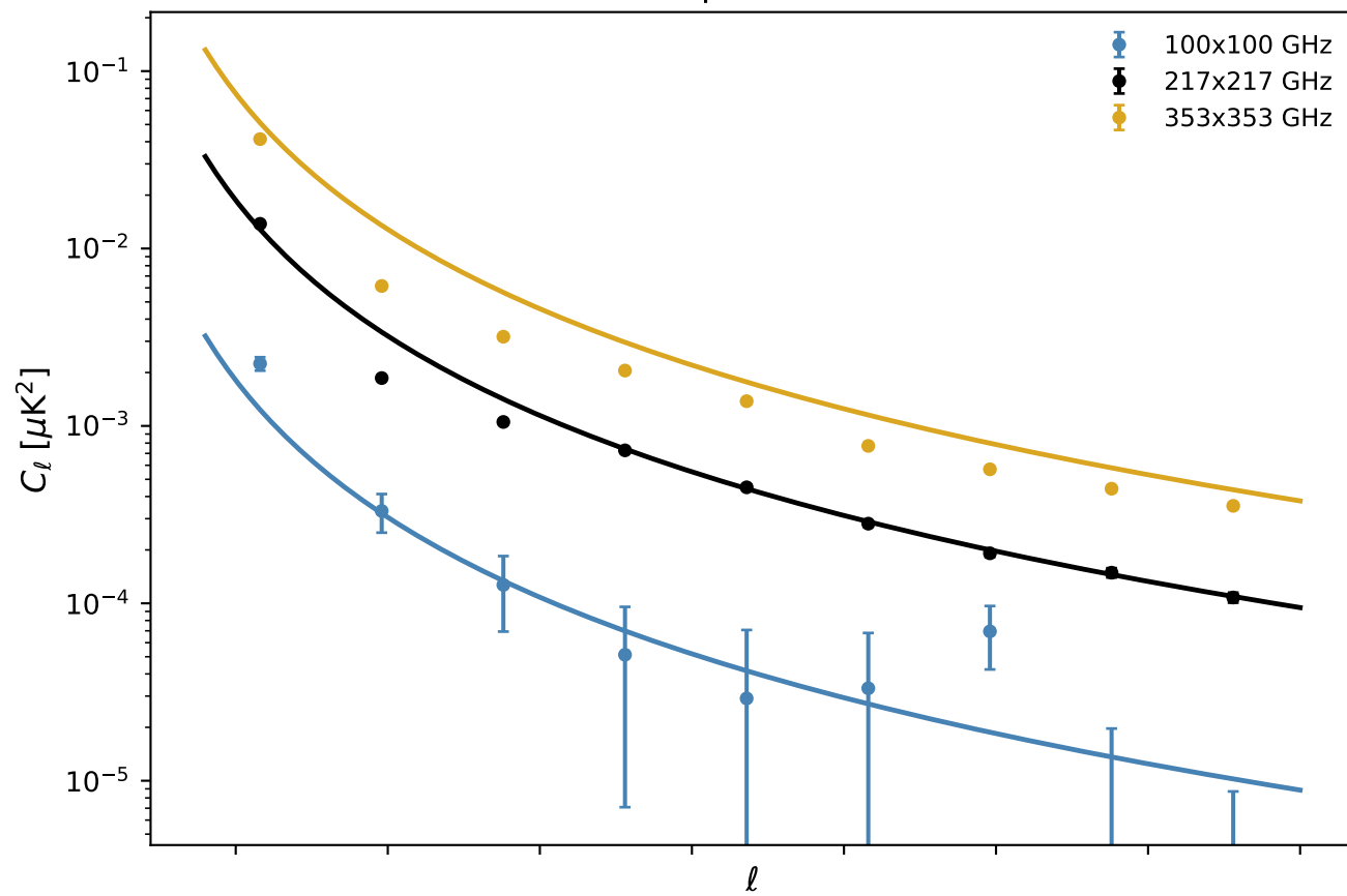
Cross-spectra — EE
