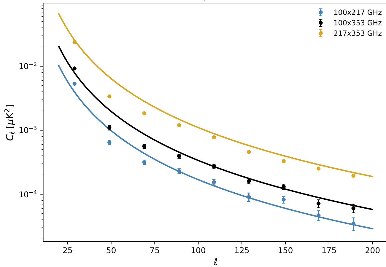
Cross-spectra — EE
