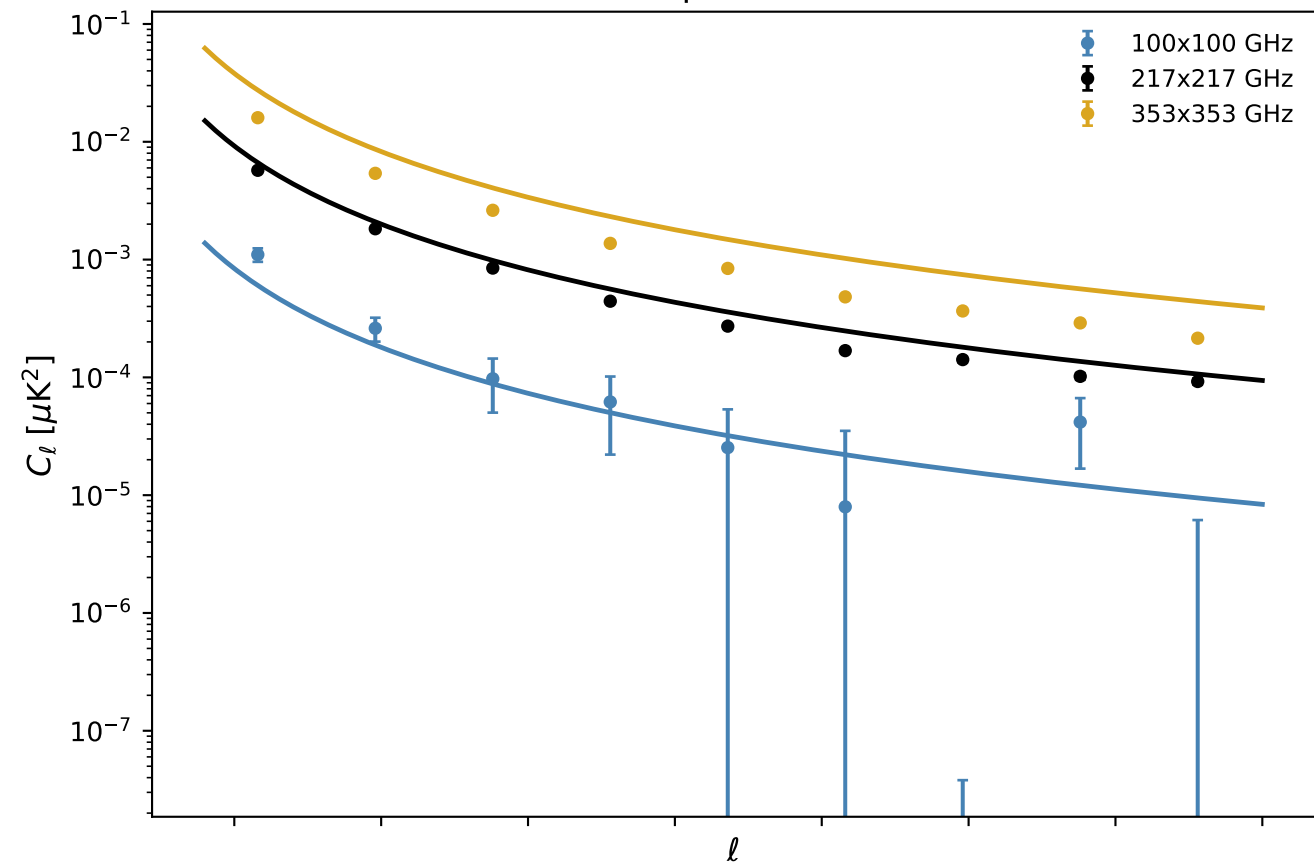
Cross-spectra — BB
