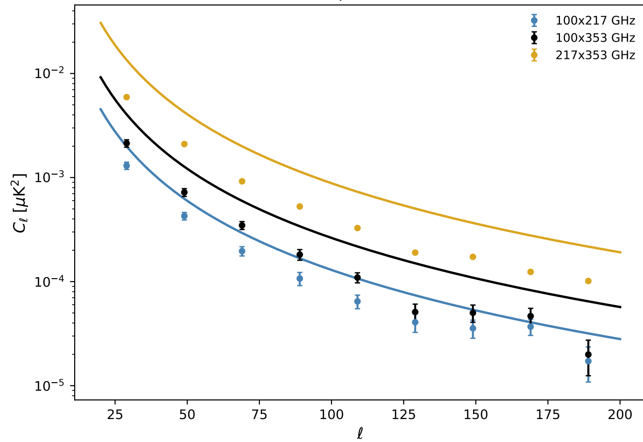
Cross-spectra — BB
