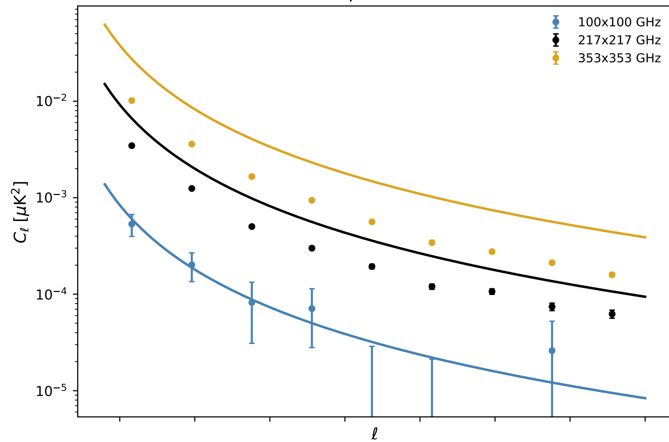
Cross-spectra — BB
