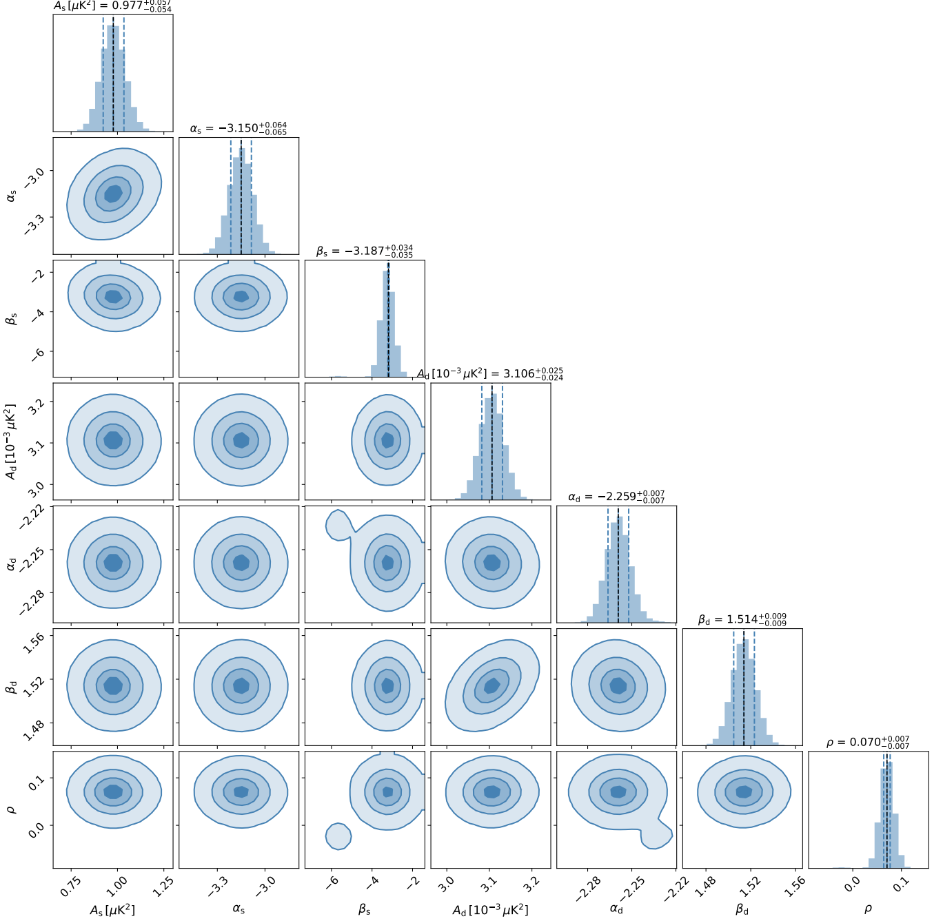
Figure 6: Corner plot showing posterior distributions for synchrotron and dust model parameters from MCMC fitting of observational EE mode data with bin width \Delta\ell = 20 . The plot displays parameter constraints and correlations obtained from power-law model fitting to the real sky maps with wider binning.
