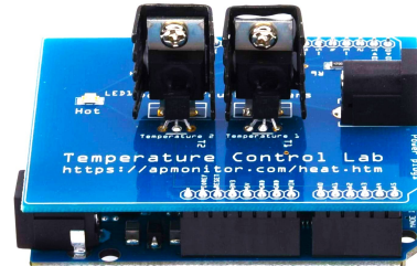
Fig II.1: Planta TCLab
