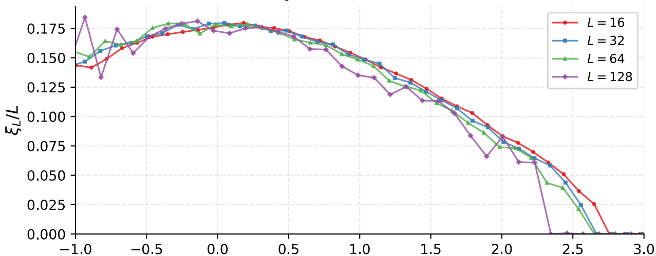
Colapso FSS — \xi_L/L | Metropolis T_c = 2.2730 , \nu = 0.975
