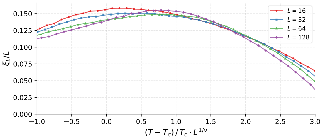
Colapso FSS — \xi_L/L | Wolff T_c = 2.2720 , \nu = 0.985
