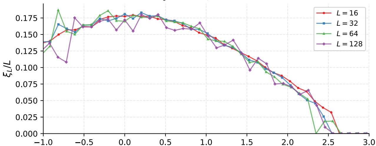
Colapso FSS — \xi_L/L | Glauber T_c = 2.2690 , \nu = 0.995
