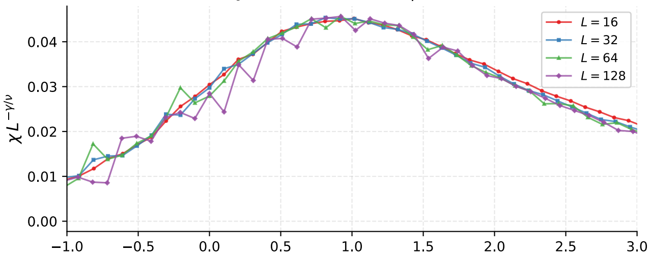
Colapso FSS — \chi | Glauber T_c = 2.2690 , \nu = 0.995 , \gamma = 1.760
