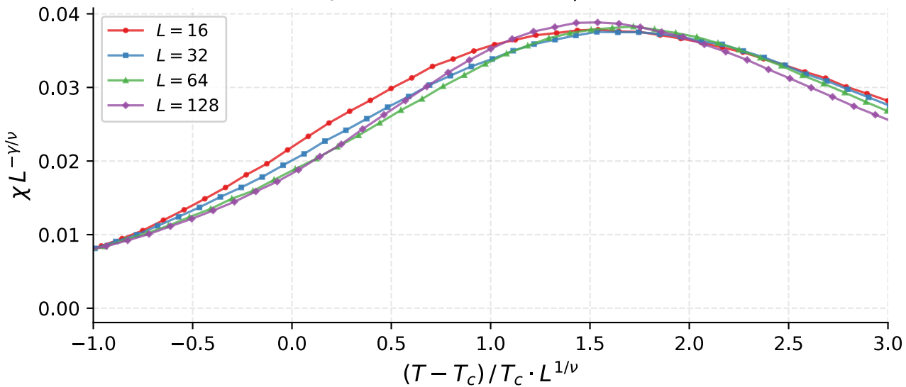
Colapso FSS — \chi | Wolff T_c = 2.2720 , \nu = 0.985 , \gamma = 1.740
