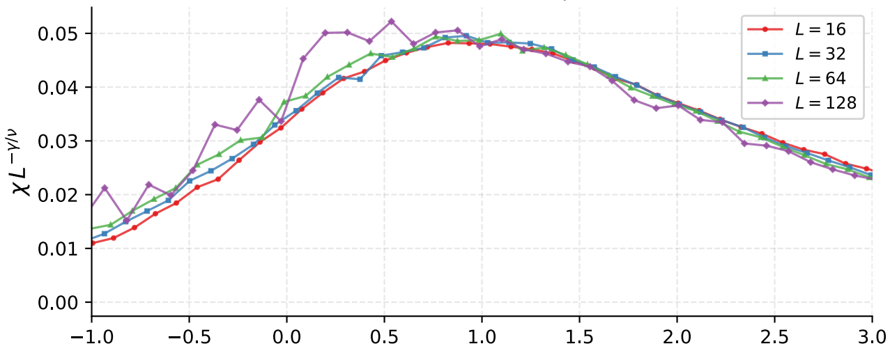
Colapso FSS — \chi | Metropolis T_c = 2.2730 , \nu = 0.975 , \gamma = 1.700
