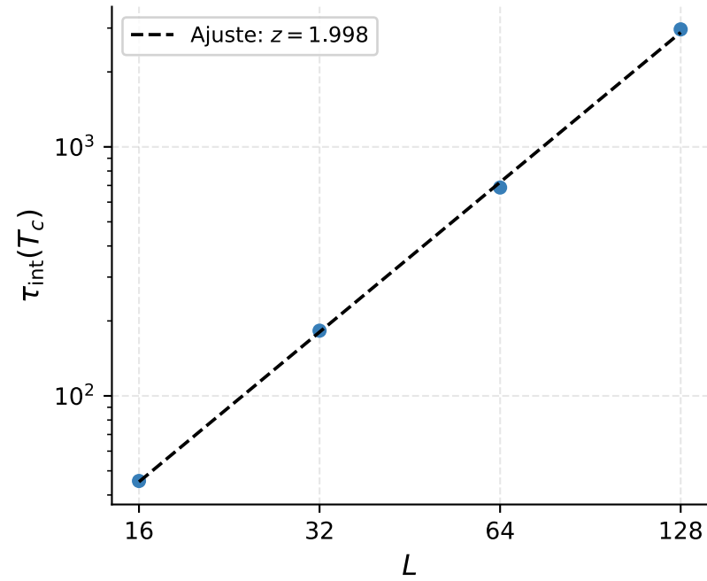
\tau_{\text{int}}(T_c) vs L — Metropolis
