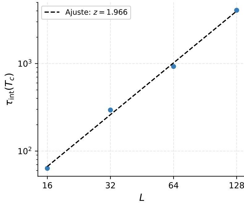
\tau_{\text{int}}(T_c) vs L — Glauber
