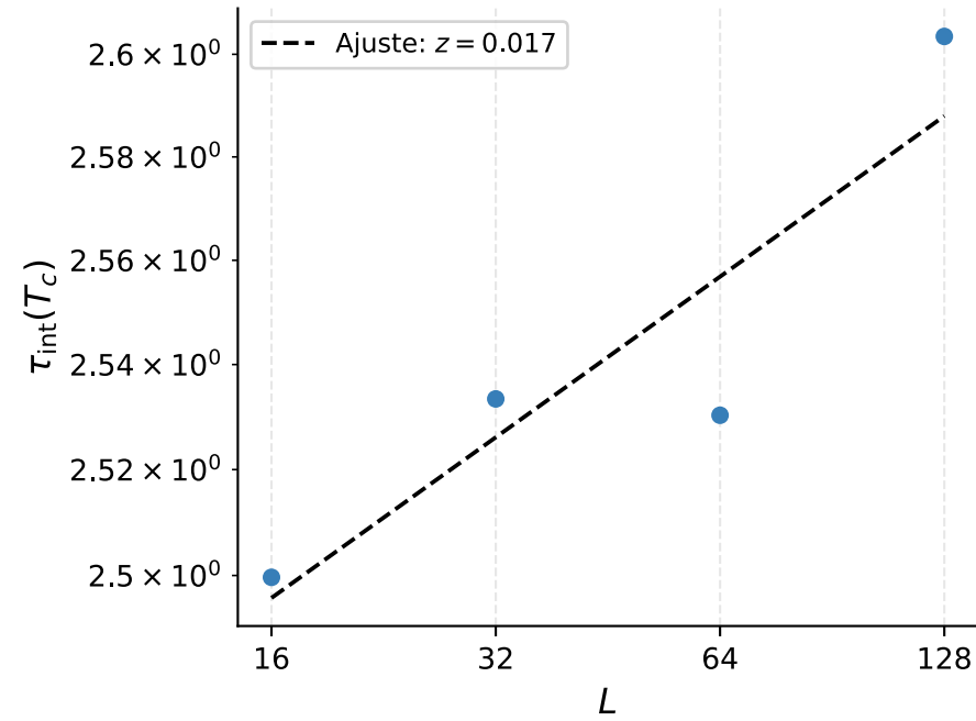
\tau_{\text{int}}(T_c) vs L — Wolff
