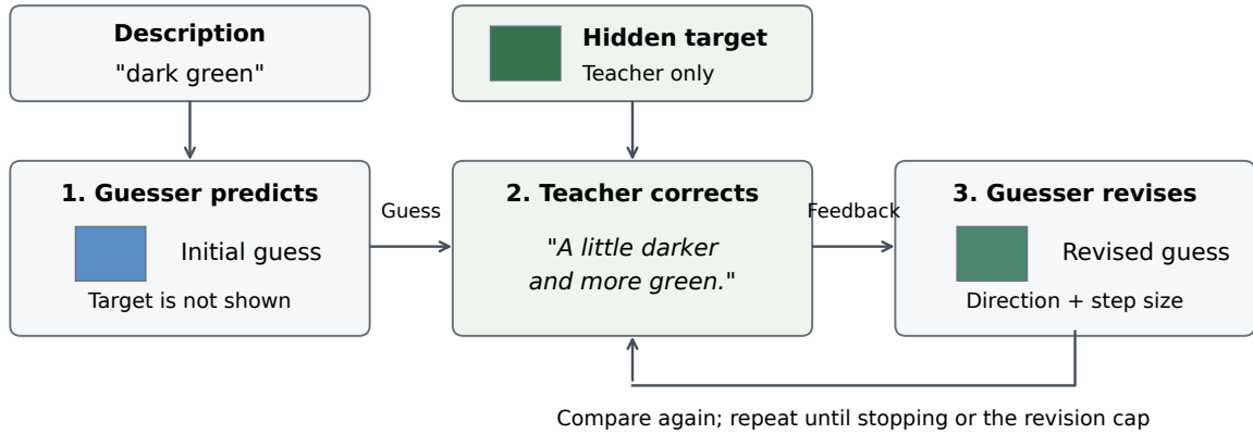
Figure 1: The ColorRef reference game, illustrated with dark green . The guesser sees the description and predicts a color; the teacher knows the hidden target and gives a correction. The revised guess becomes the state for the next exchange. A message such as a little darker and more green raises two questions: does the receiver move in the requested directions, and does it take an appropriate step? Swatches and wording here are schematic examples, not measured model responses.
