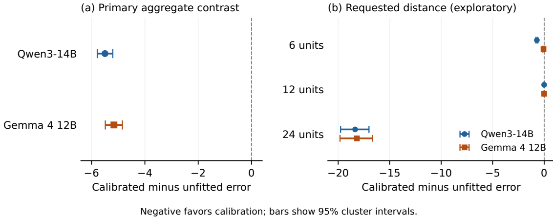
Figure 2: Receiver-specific calibration reduces displayed target error relative to the fixed unfitted quantifier rule for both models (left). Exploratory distance breakdowns concentrate the benefit at 24-unit targets (right). Bars show 95% starting-color cluster percentile intervals; each model covers the same 128 starting colors, with 2,098 Qwen and 2,081 Gemma common parsed quartets. These are within-model contrasts, not a paired between-model test. The panels use different horizontal scales. Values are reproduced from reported rounded estimates.
