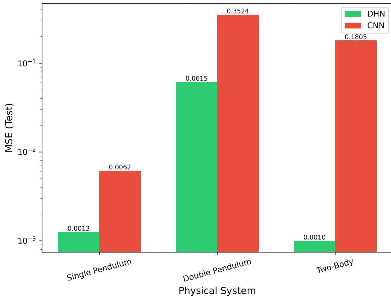
Diff-Init (Out-of-Distribution)
