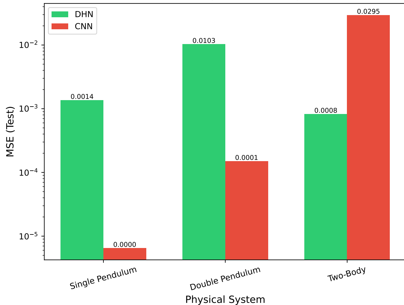
Same-Init (In-Distribution)
