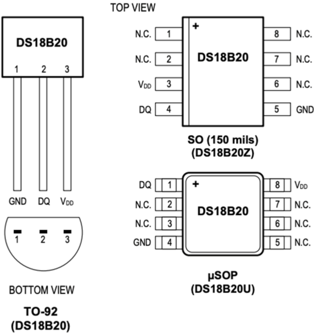
Figura 5: PIN OUT DS18B20
