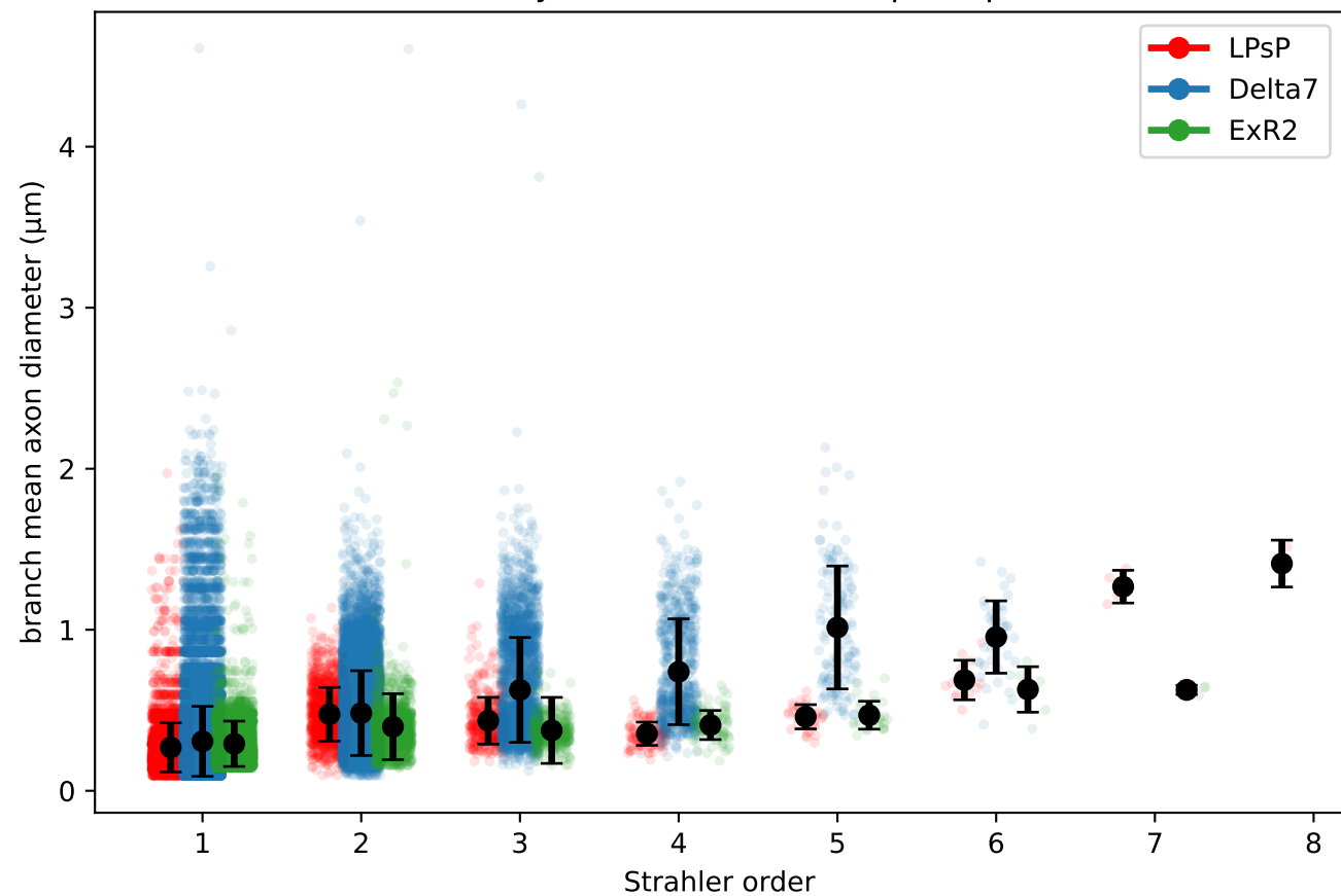
Axon diameter by Strahler order (one point per branch)
