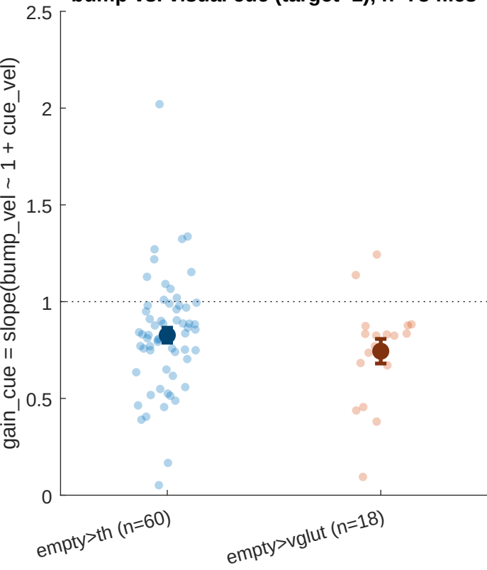
bump vs. visual cue (target=1), n=78 flies
