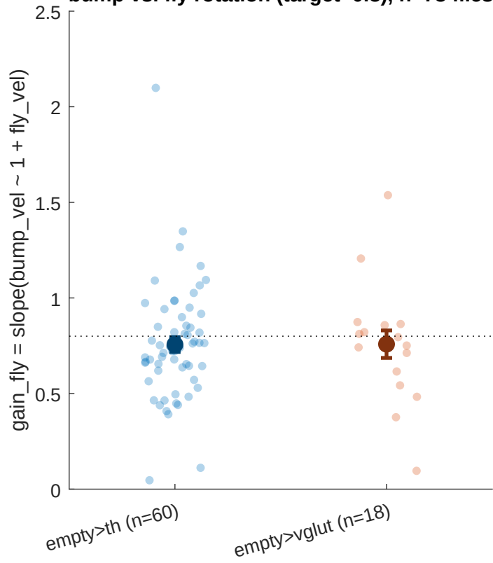
bump vs. fly rotation (target=0.8), n=78 flies
