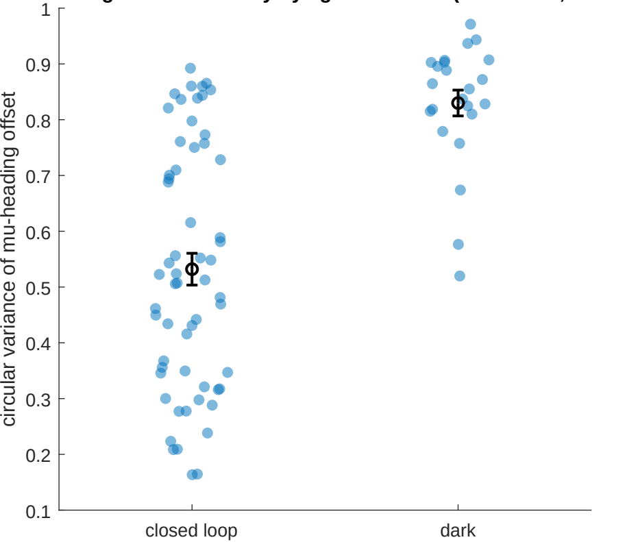
mu-heading offset variability by light condition (n=82 trials, \rho>0.1 )
