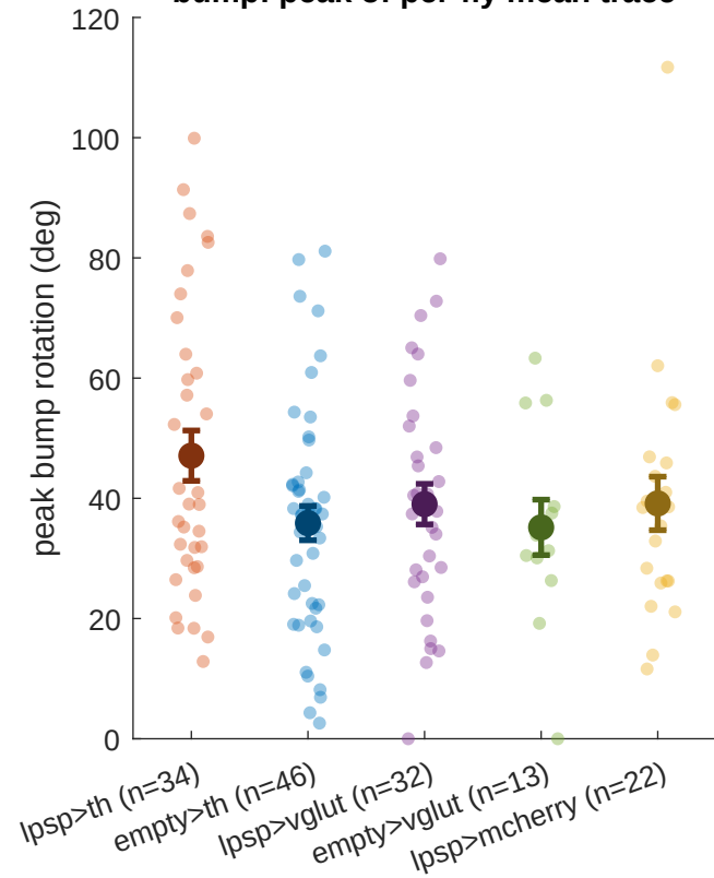
bump: peak of per-fly mean trace
