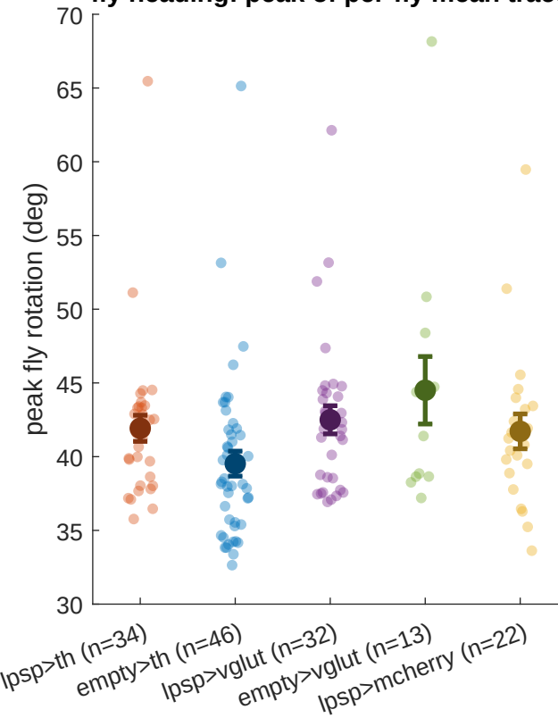
fly heading: peak of per-fly mean trace
