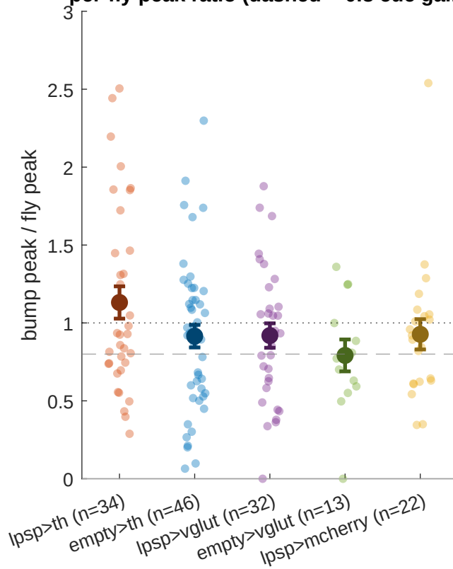
per-fly peak ratio (dashed = 0.8 cue gain)
