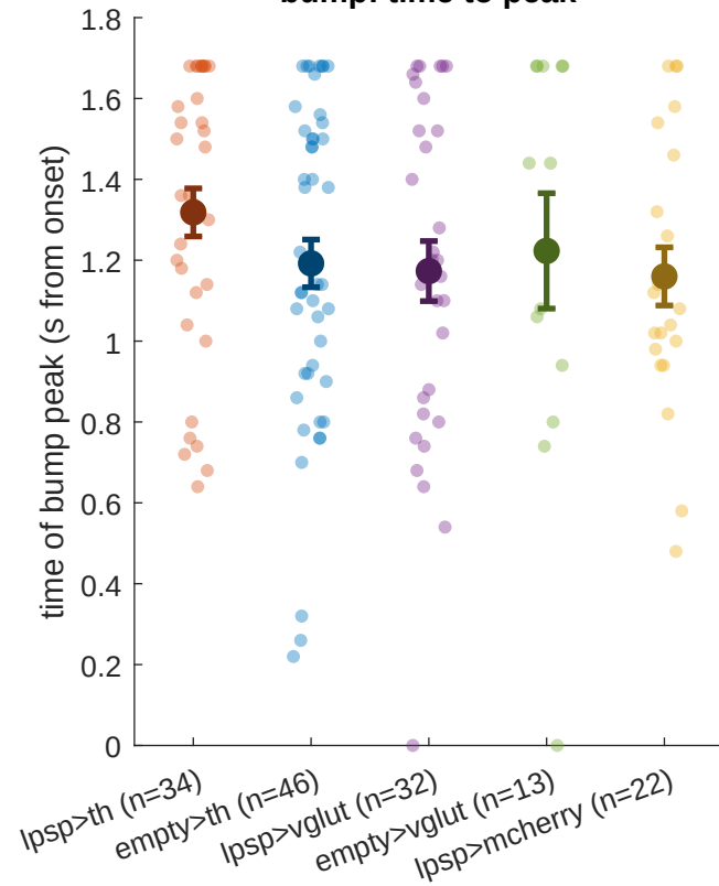
bump: time to peak
