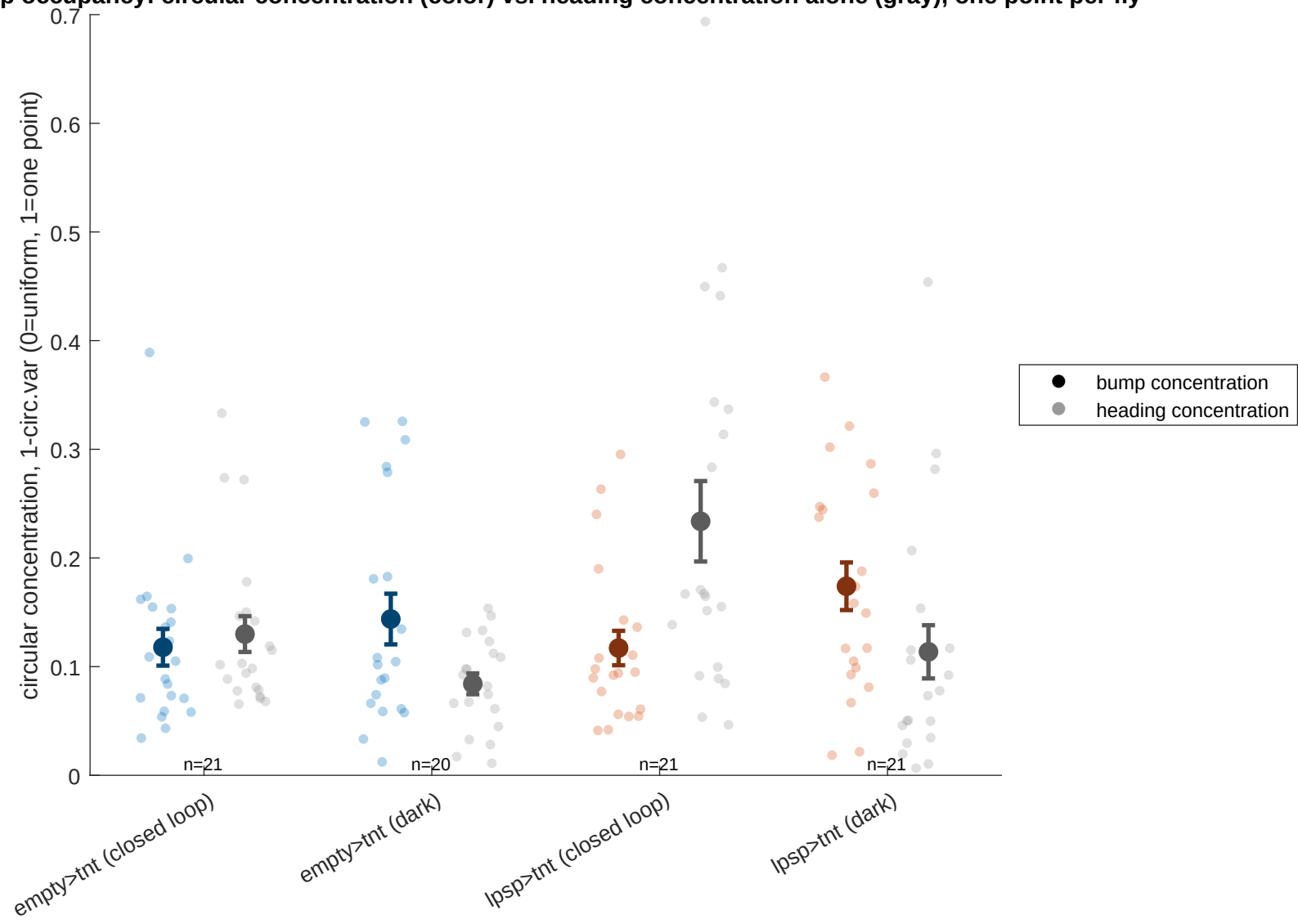
bump occupancy: circular concentration (color) vs. heading concentration (gray), one point per fly
