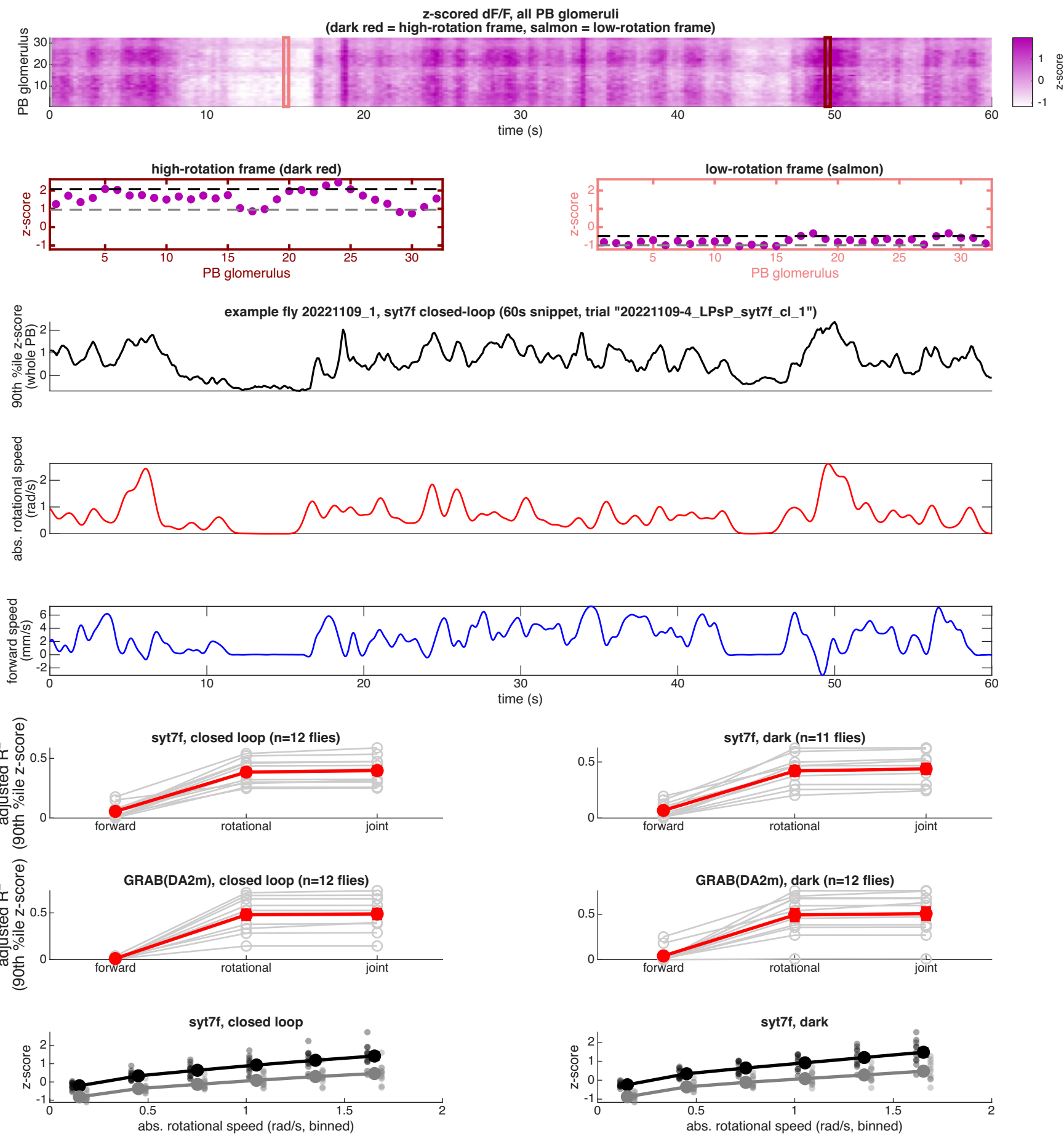
Figure 2a: PB dF/F encoding of forward/rotational speed, syt7f and GRAB(DA2m) (syt7f example)
