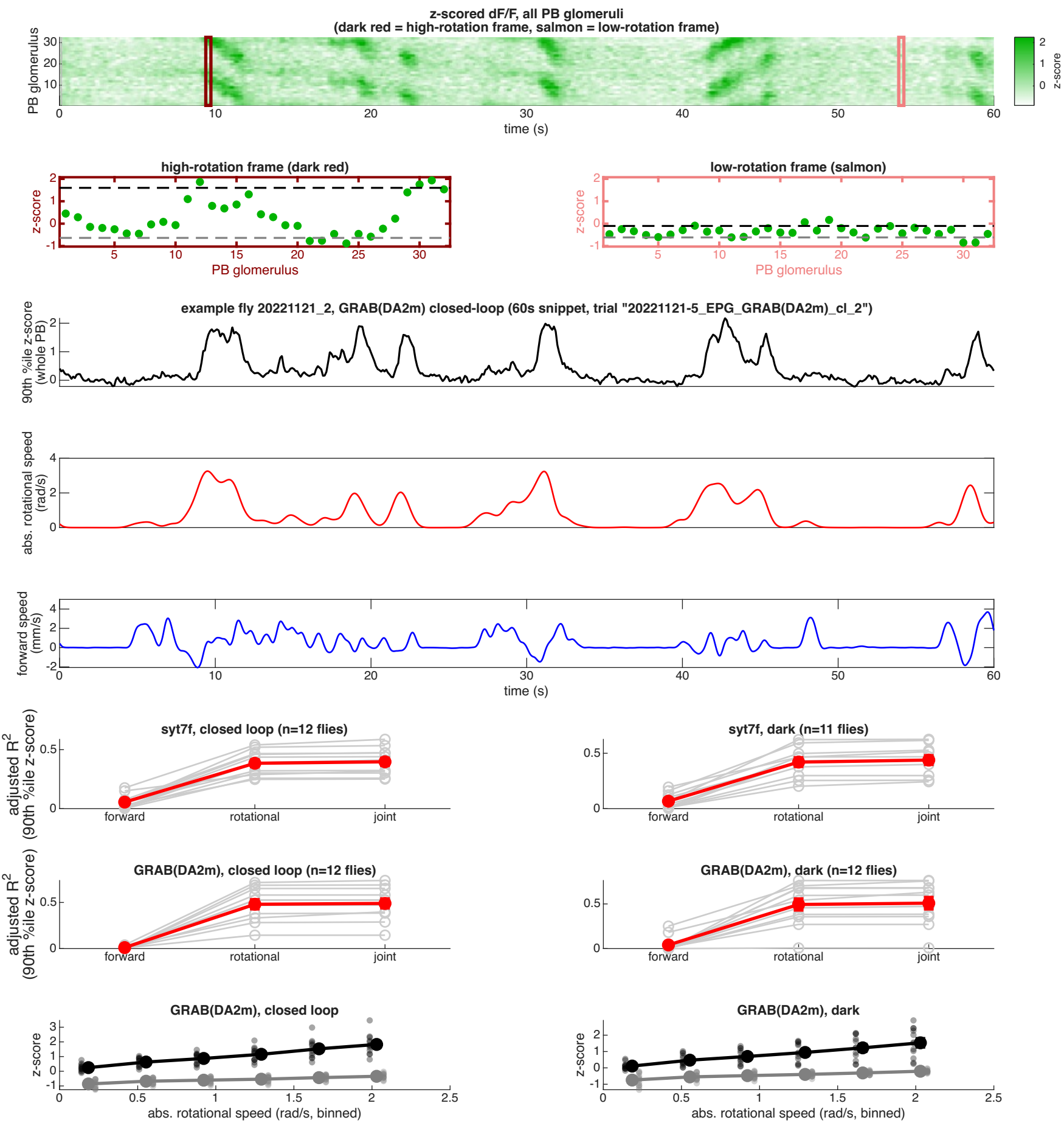
Figure 2b: PB dF/F encoding of forward/rotational speed, syt7f and GRAB(DA2m) (GRAB(DA2m) example)
