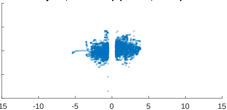
syt8m, closed loop (n=4974, r=0.26)
