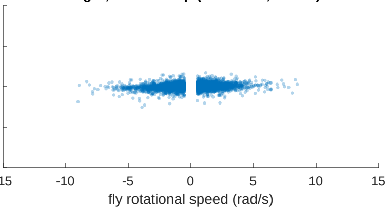
dLight, closed loop (n=677470, r=0.19)
