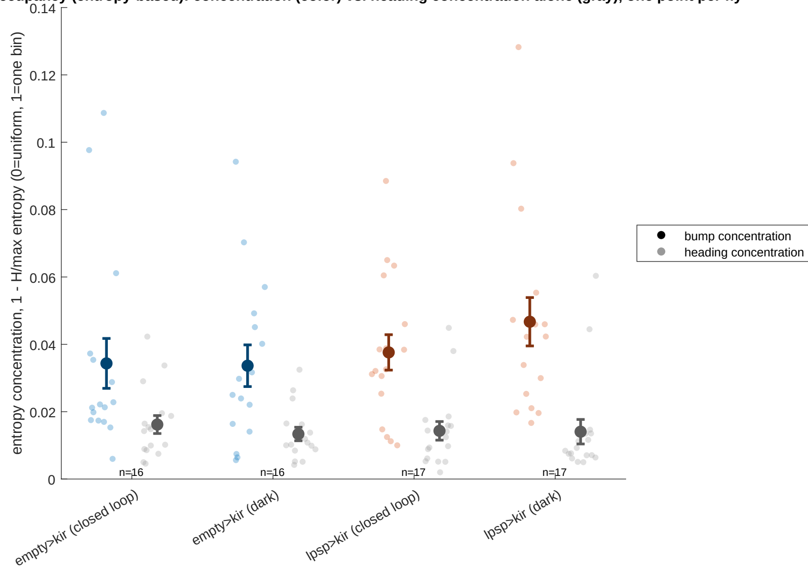
mp occupancy (entropy-based): concentration (color) vs. heading concentration alone (gray), one point per fly
