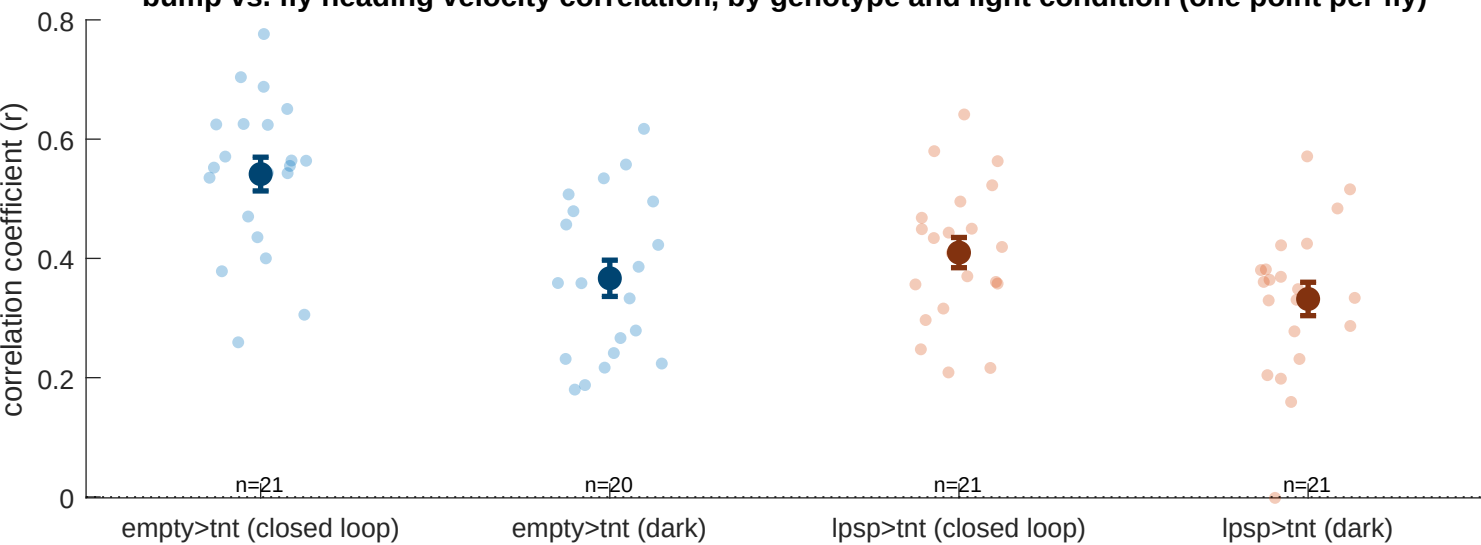
bump vs. fly heading velocity correlation, by genotype and light condition (one point per fly)
