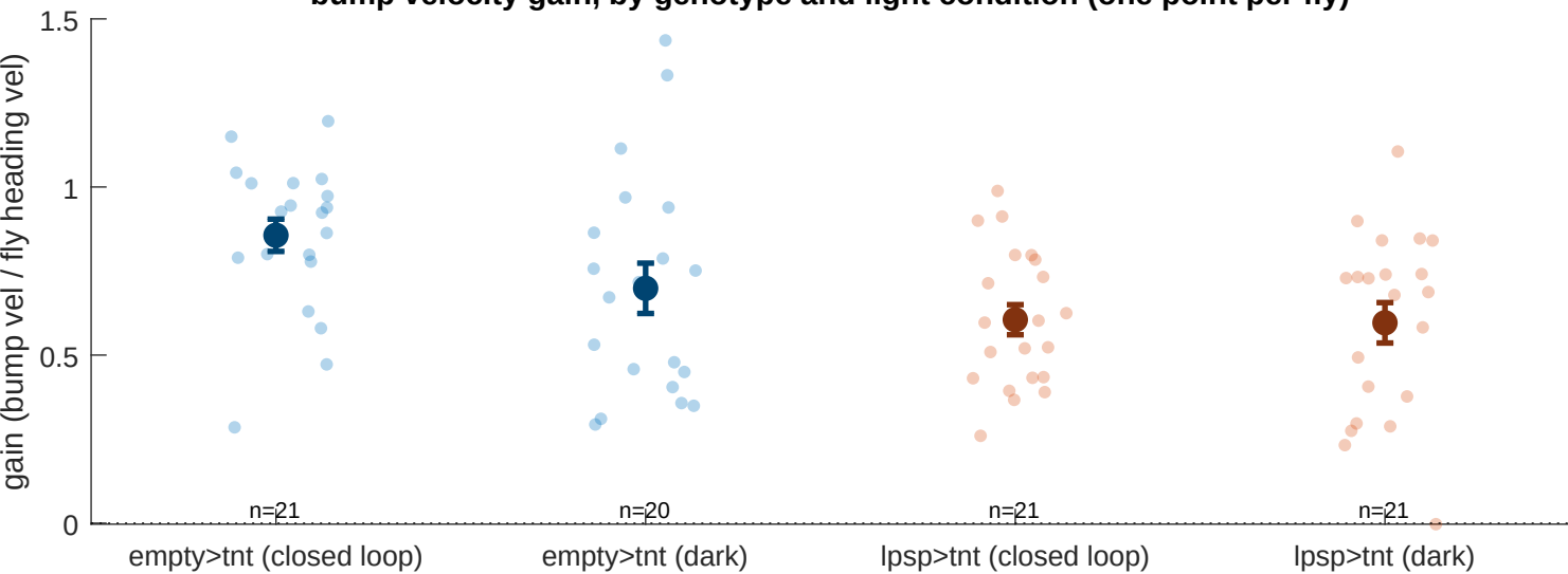
bump velocity gain, by genotype and light condition (one point per fly)
