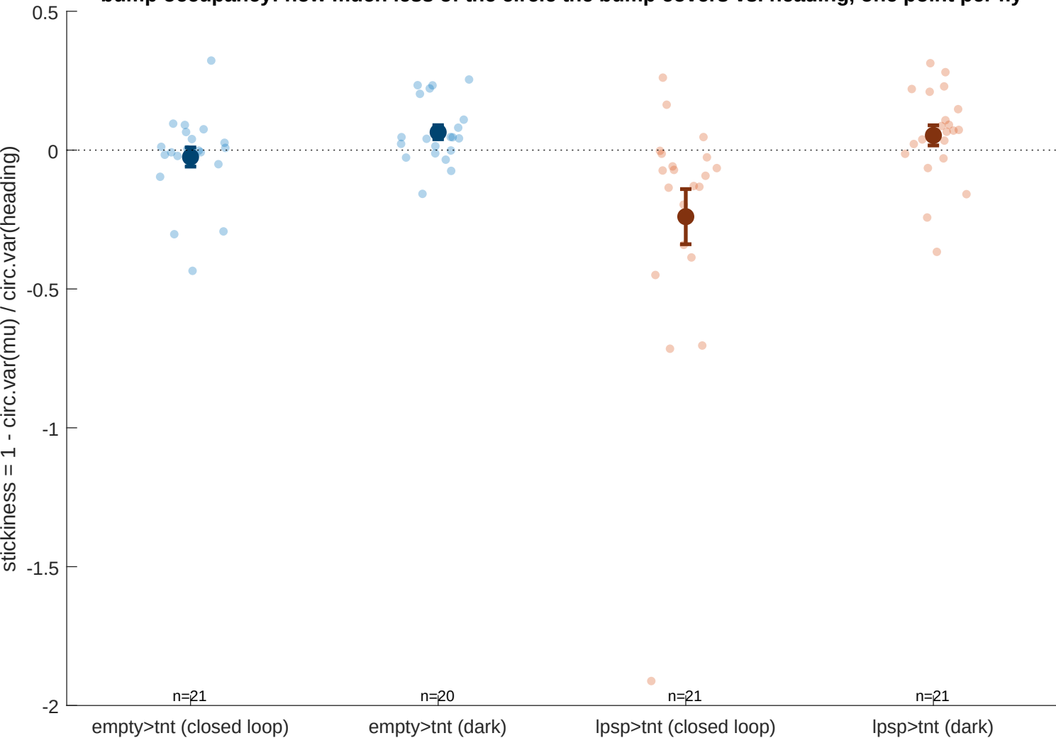
bump occupancy: how much less of the circle the bump covers vs. heading, one point per fly
