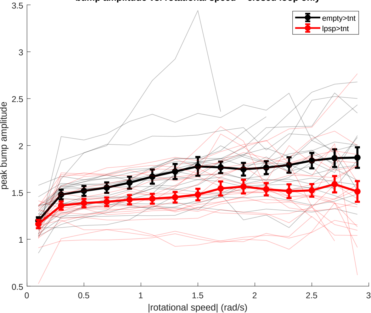
bump amplitude vs. rotational speed -- closed loop only
