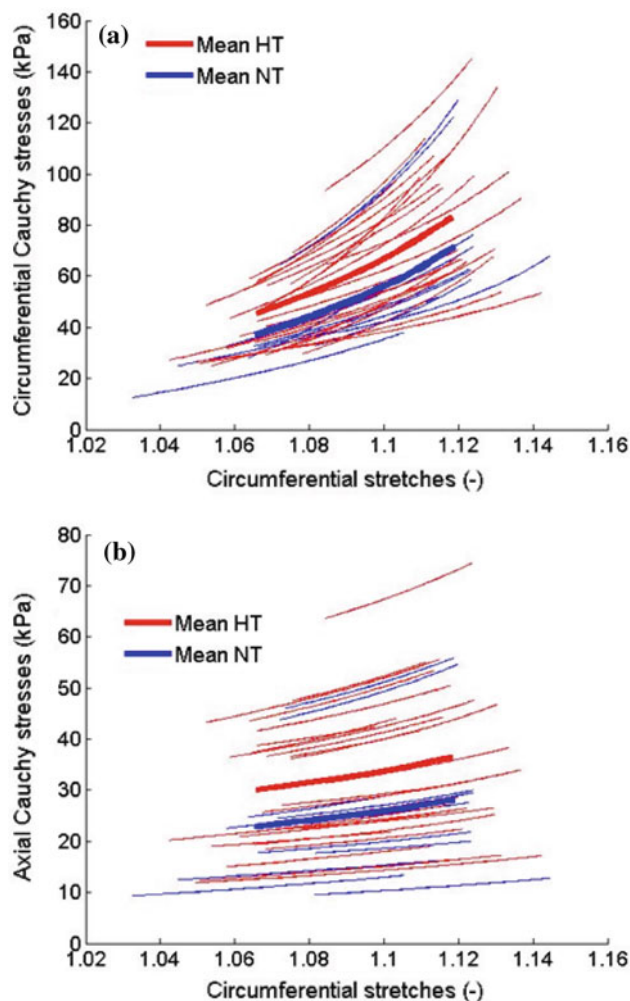
Fig. 7 a Circumferential and b axial Cauchy stresses as a function of circumferential stretches, expressed at the outer media ( r_m ), for both the 25 hypertensive patients (HT) and the subgroup of 11 normotensive subjects (NT) matched for age. HT are displayed in red and NT in blue, with the respective mean values shown by the darker solid lines. Mean circumferential and axial stresses (expressed at the mean stretch of the outer medial location) were, respectively, 19 and 32% higher in HT compared to NT subjects
