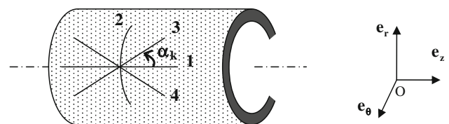
Fig. 2 Schema of the four collagen-fiber families, with the diagonal fibers characterized by angle \alpha relative to the axial direction in a cylindrical arterial segment
