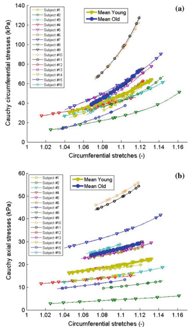
Fig. 5 a Circumferential and b axial Cauchy stresses as a function of circumferential stretches, expressed at the outer media r_m , for all 16 normotensive subjects. The seven youngest subjects (from 21 to 42 years old) are denoted by inverted triangles ( \nabla ) and the nine oldest ones (from 53 to 64 years old) by circles ( \circ ). The respective mean values are shown by darker solid lines : the “Young” group in ochre and the “Old” group in blue. Mean circumferential and axial stresses (expressed at the approximate mean stretch of the outer medial location) were, respectively, 14 and 37% higher in older compared to younger subjects. For display purposes, one point in twenty was plotted for clarity, although computations were performed on the full data sets
