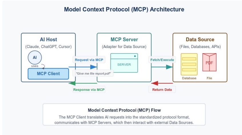
Figura 2.7: Diagrama de la arquitectura MCP. Fuente: https://newsletter.diamant-ai.com/p/model-context-protocol-mcp-explained
