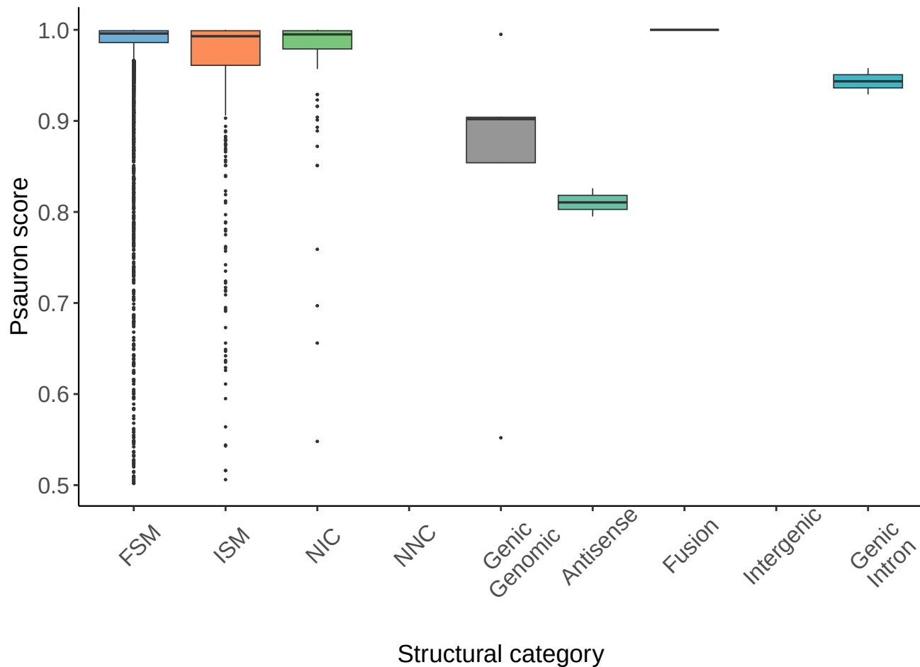
Psaaron score per structural category
