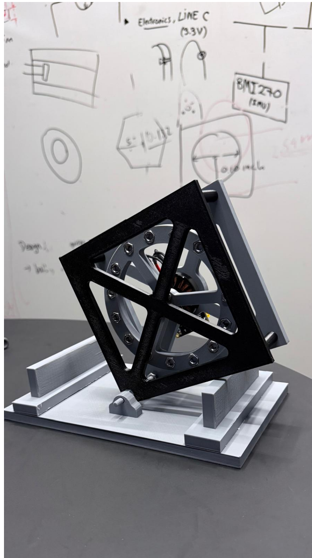
Figure 8: The single-face prototype rig as built: one reaction wheel driven by a brushless motor on a diagonally-mounted printed plate, pivoting on a corner bearing against a printed base with hard stops. This is the article on which the plant parameters of Table 7 are measured and the single-axis controller of Section 7 is validated before the three-axis build. The drawing set is given in Appendix B.3.
