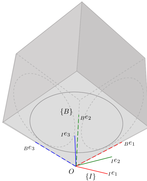
Figure 7: Body frame \{B\} and inertial frame \{I\} of the three-axis cube, both originated at the corner contact point O . The body axes B e_1, B e_2, B e_3 coincide with the wheel spin axes e_i of Table 9, each directed outward from O along a cube edge; \{I\} is fixed in space and coincides with \{B\} at the corner-up equilibrium, so R = \mathbb{I} there.
