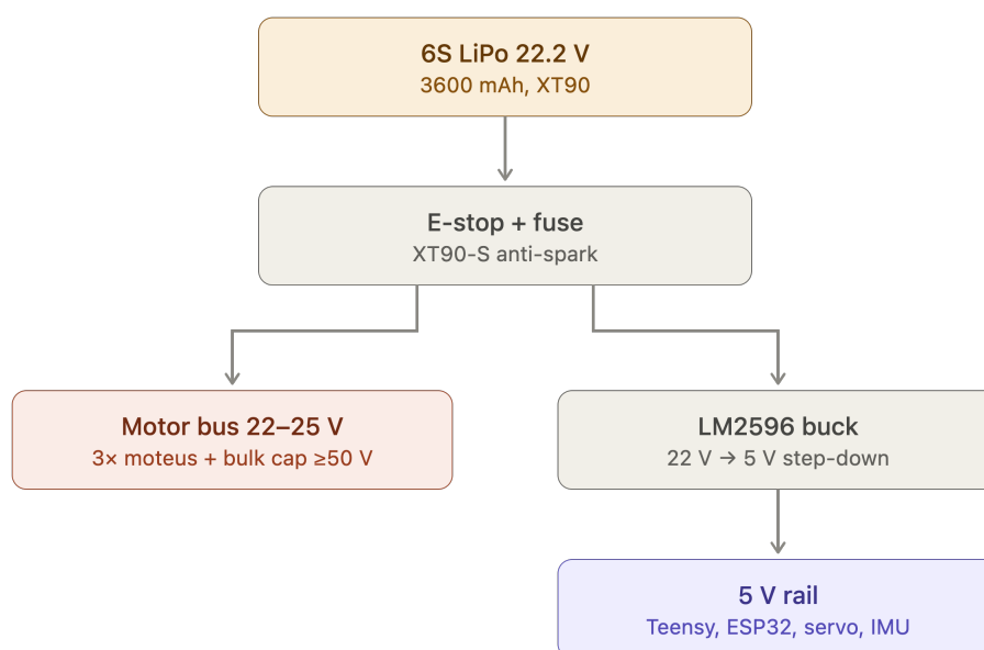
Figure 13: Power distribution tree. A single 6S pack feeds the motor bus directly and the 5 V logic rail through a buck converter, both behind a common E-stop and fuse.
