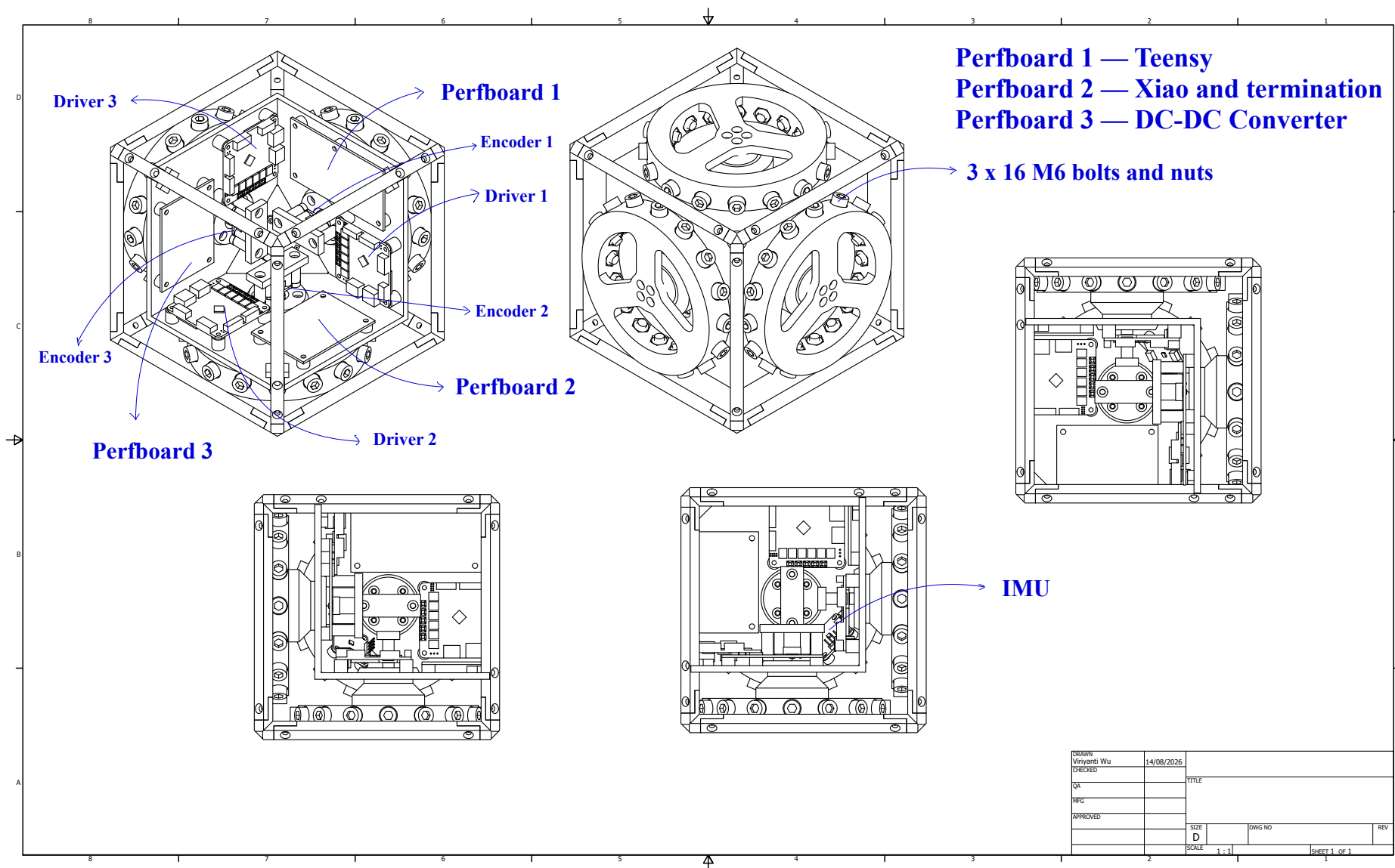
Figure 16: General-assembly drawing of the three-axis cube — the final released design of the flight article — sheet 1 of 1 at 1:1, with the electronics package called out per Section 6.6. Upper left: isometric cutaway of the inner structure, labelling the three motor drivers (Driver 1–3), the three encoder boards (Encoder 1–3) and the three perfboard assemblies (Perfboard 1: Teensy flight controller; Perfboard 2: Xiao and termination; Perfboard 3: DC-DC converter). Upper centre: isometric view of the closed assembly, showing the three orthogonal reaction-wheel modules through the open frame faces and the 3 \times 16 M6 ballast bolt-and-nut set. Right: front elevation in section of a single motor/wheel module, locating the IMU on the inner structure. Lower left and lower centre: front orthographic views of two face modules, giving the motor bolt circle and the corner fastener pattern of Table 17.
