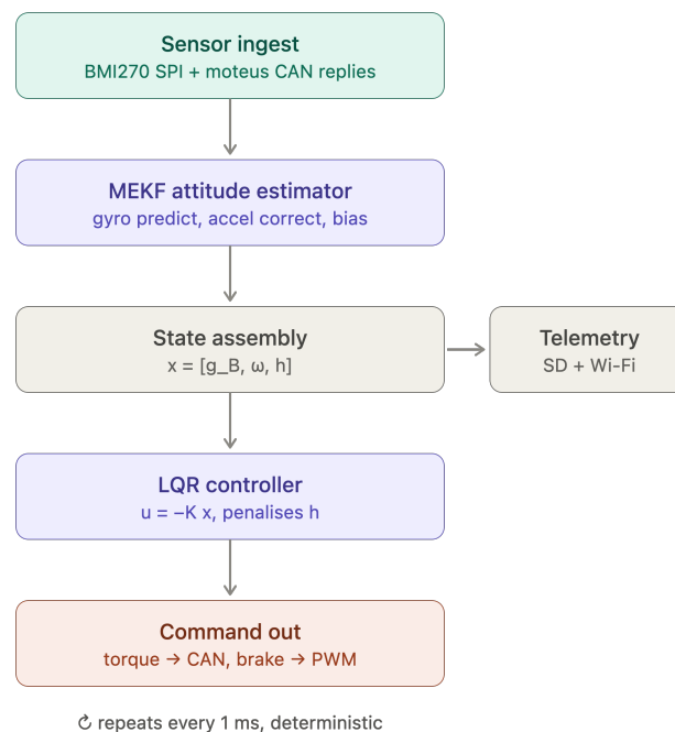
Figure 14: Teensy 4.1 control-loop software pipeline. The estimator and controller stages implement the design of Section 7.1; telemetry is a side-branch off the control path.
