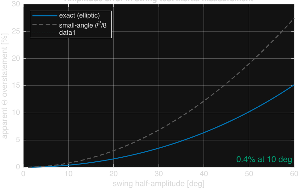
Amplitude error in swing-test inertia measurement
