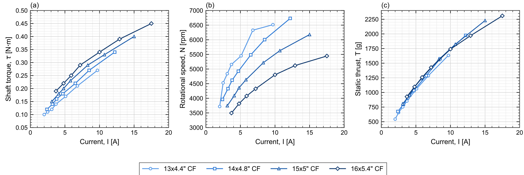
Figure 1. Measured torque, rotational speed and static thrust against motor current for four carbon-fibre propellers on a single T-MOTOR unit. Symbols are measured points at throttle settings of 50, 55, 60, 65, 75, 85 and 100 %; lines join successive points and are not fits. Static bench test data, manufacturer supplied. The 16x5.4 in. run reached the motor thermal limit at 100 % throttle.
