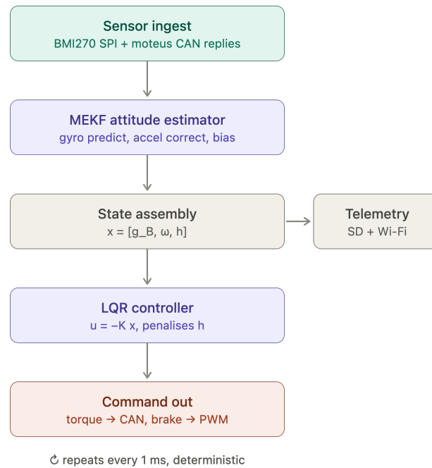
Figure 8: Teensy 4.1 control-loop software pipeline. The estimator and controller stages implement the design of Section 4.4; telemetry is a side-branch off the control path.
