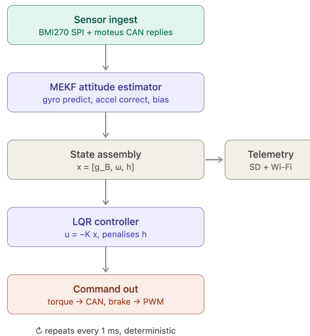
Figure 10: Teensy 4.1 control-loop software pipeline. The estimator and controller stages implement the design of Section 7.1; telemetry is a side-branch off the control path.
