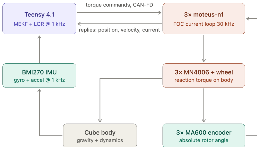
Figure 7: System architecture and control loop. Blue: processing; green: sensing; orange: actuation. Rates shown are the design targets of Section 7.
