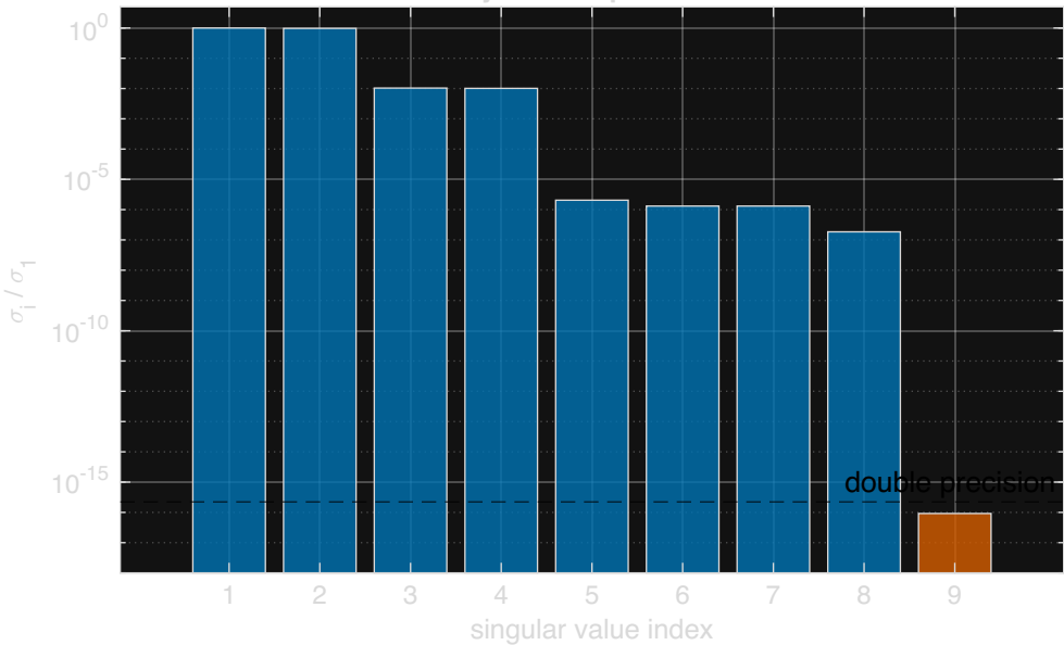
Controllability matrix spectrum: rank 8 of 9
