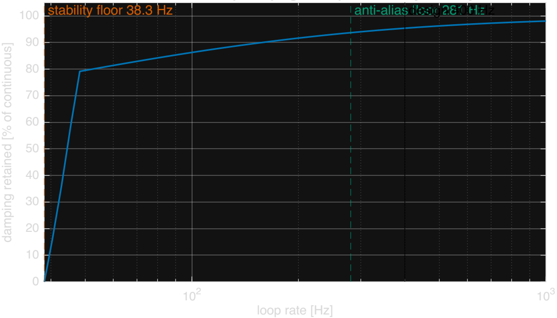
Discrete closed-loop damping vs loop rate, one-cycle delay
