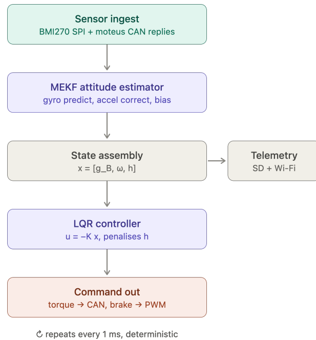
Figure 10: Teensy 4.1 control-loop software pipeline. The estimator and controller stages implement the design of Section 4.4; telemetry is a side-branch off the control path.
