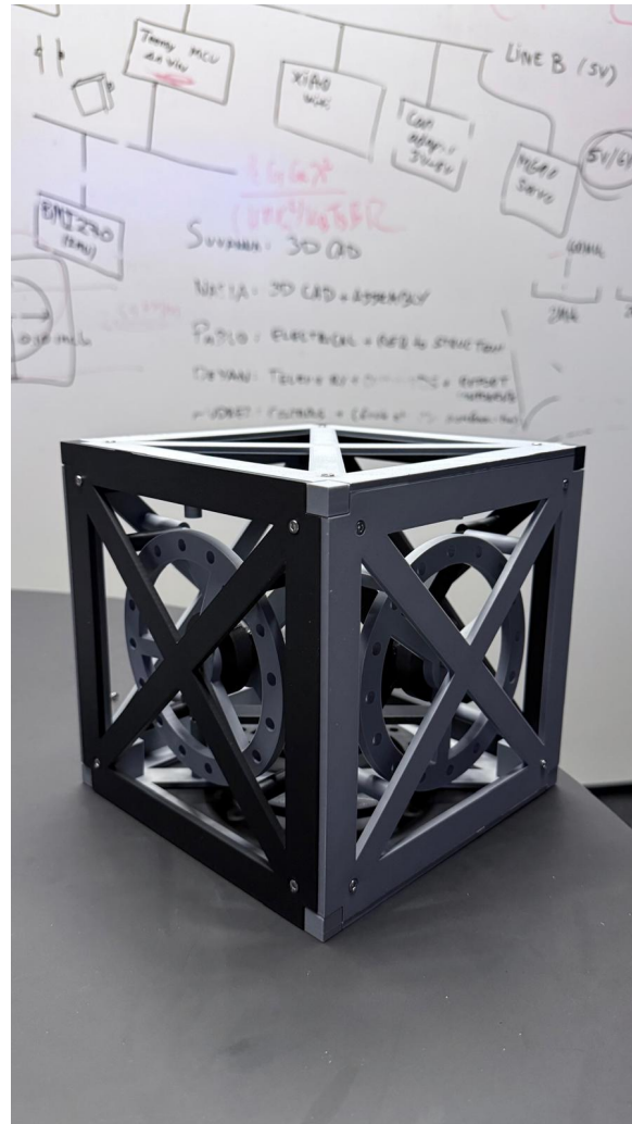
Figure 10: Printed concept prototype of the three-axis cube frame, showing the X-braced outer faces and the three orthogonal reaction-wheel modules carried by the inner structure. This article validates the two-part architecture and the internal packaging only: it is not the final design. Wheel geometry and the frame edge length L remain subject to the sizing closure of Sections 5.2 and 5.3, so its mass properties do not represent the budgeted values. The frozen design's general-assembly drawing is given in Figure 17 of Appendix B.4.
