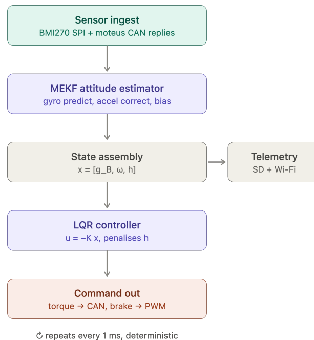
Figure 12: Teensy 4.1 control-loop software pipeline. The estimator and controller stages implement the design of Section 7.1; telemetry is a side-branch off the control path.
