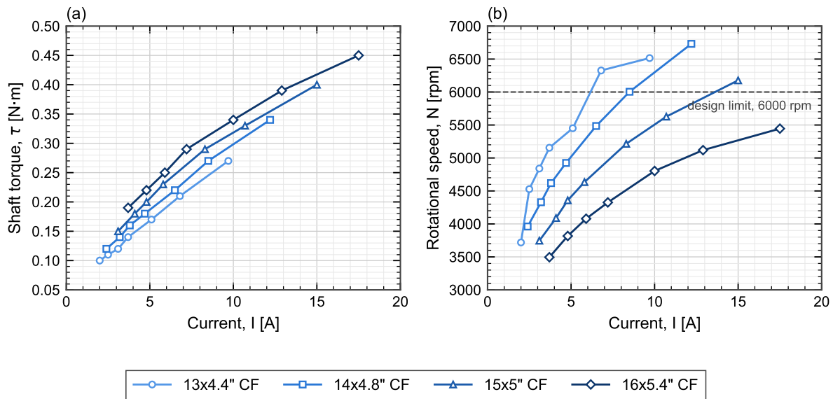
Figure 3: Measured MN4006 (a) shaft torque and (b) rotational speed against phase current, for one motor driving four different loads. Symbols are measured points at throttle settings of 50, 55, 60, 65, 75, 85 and 100 %; lines join successive points and are not fits. The dashed line in (b) is the 6000rpm reaction-wheel design ceiling of Section 5.2. Loads shown are propellers, not reaction wheels: the curves characterise the motor , and the load-dependent spread between them does not carry over to this application. Manufacturer static bench data; the heaviest load reached the motor thermal limit at 100 % throttle.
