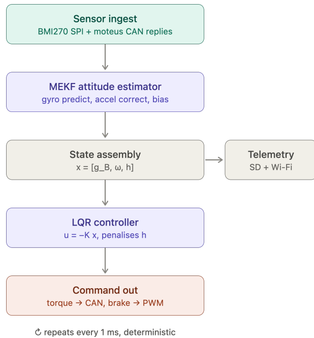
Figure 5: Teensy 4.1 control-loop software pipeline. The estimator and controller stages implement the design of Section 4.4; telemetry is a side-branch off the control path.
