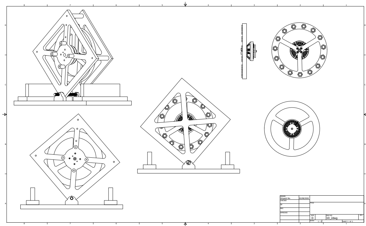
Figure 11: General-assembly drawing of the single-face (1-DoF) prototype rig, sheet 1 of 1 at 1:1. Upper left and lower left: front elevation of the rig mounted on its base, showing the diagonal plate orientation, the corner pivot and the two hard stops. Centre: side elevation through the wheel axis. Right: plan and edge views of the reaction-wheel and motor assembly, giving the spoke pattern and the ballast bolt circle used for the balancing adjustment of Section 5.3.4.
