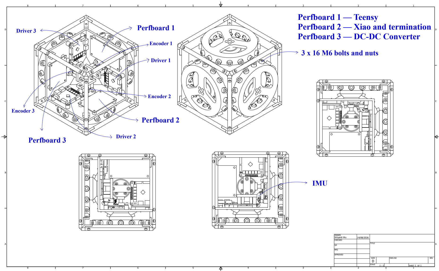
Figure 16: General-assembly drawing of the three-axis cube — the final released design of the flight article — sheet 1 of 1 at 1:1, with the electronics package called out per Section 7.6. Upper left: isometric cutaway of the inner structure, labelling the three motor drivers (Driver 1–3), the three encoder boards (Encoder 1–3) and the three perfboard assemblies (Perfboard 1: Teensy flight controller; Perfboard 2: Xiao and termination; Perfboard 3: DC-DC converter). Upper centre: isometric view of the closed assembly, showing the three orthogonal reaction-wheel modules through the open frame faces and the 3 × 6 M6 ballast bolt-and-nut set. Right: front elevation in section of a single motor/wheel module, locating the IMU in the inner structure. Lower left and lower centre: front orthographic views of two face modules, giving the motor bolt circle and the corner fastener pattern of Table 17.
