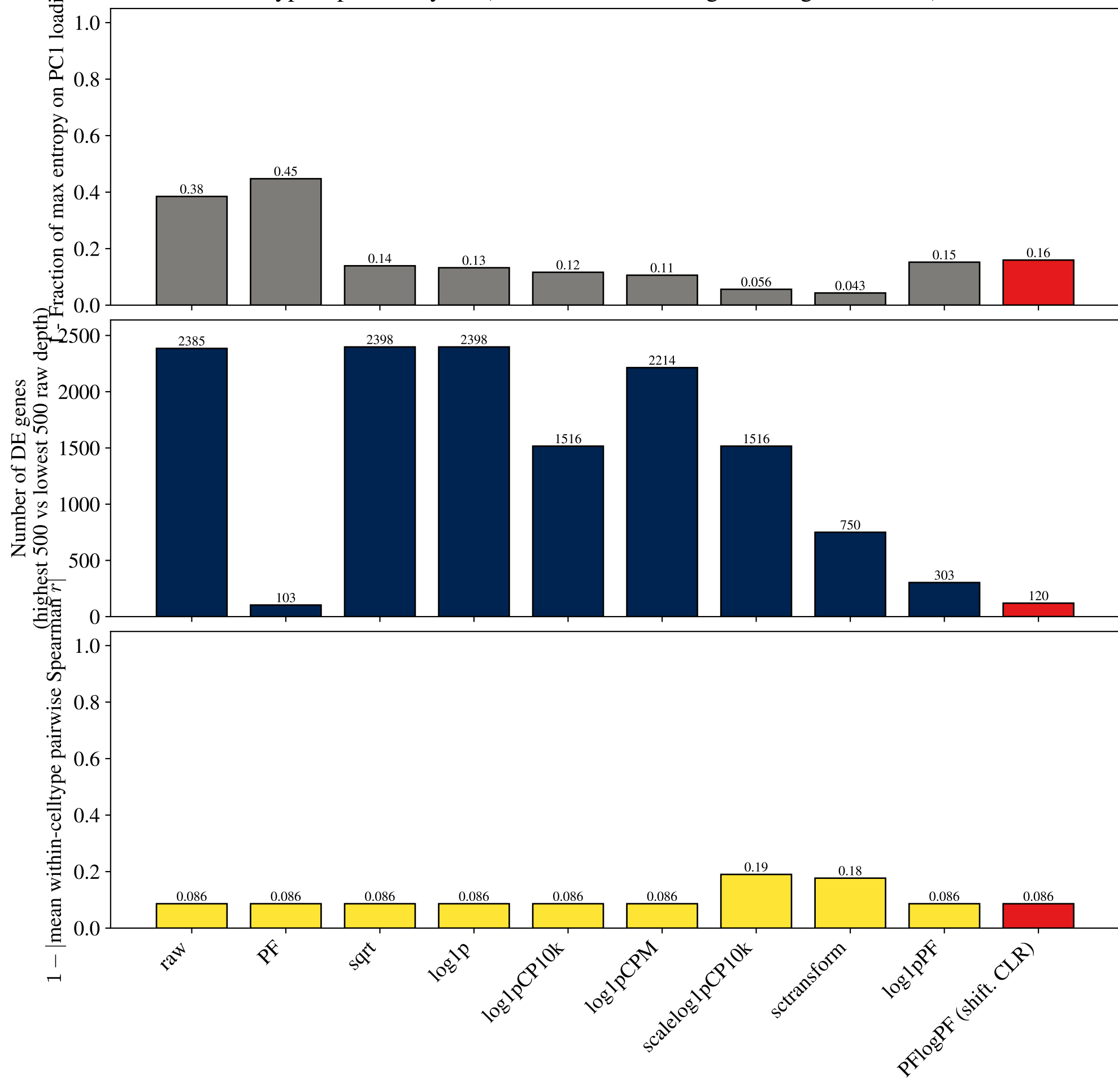
Type 2 pneumocytes (4,199 cells \times 16,541 genes, angelidis_2019)
