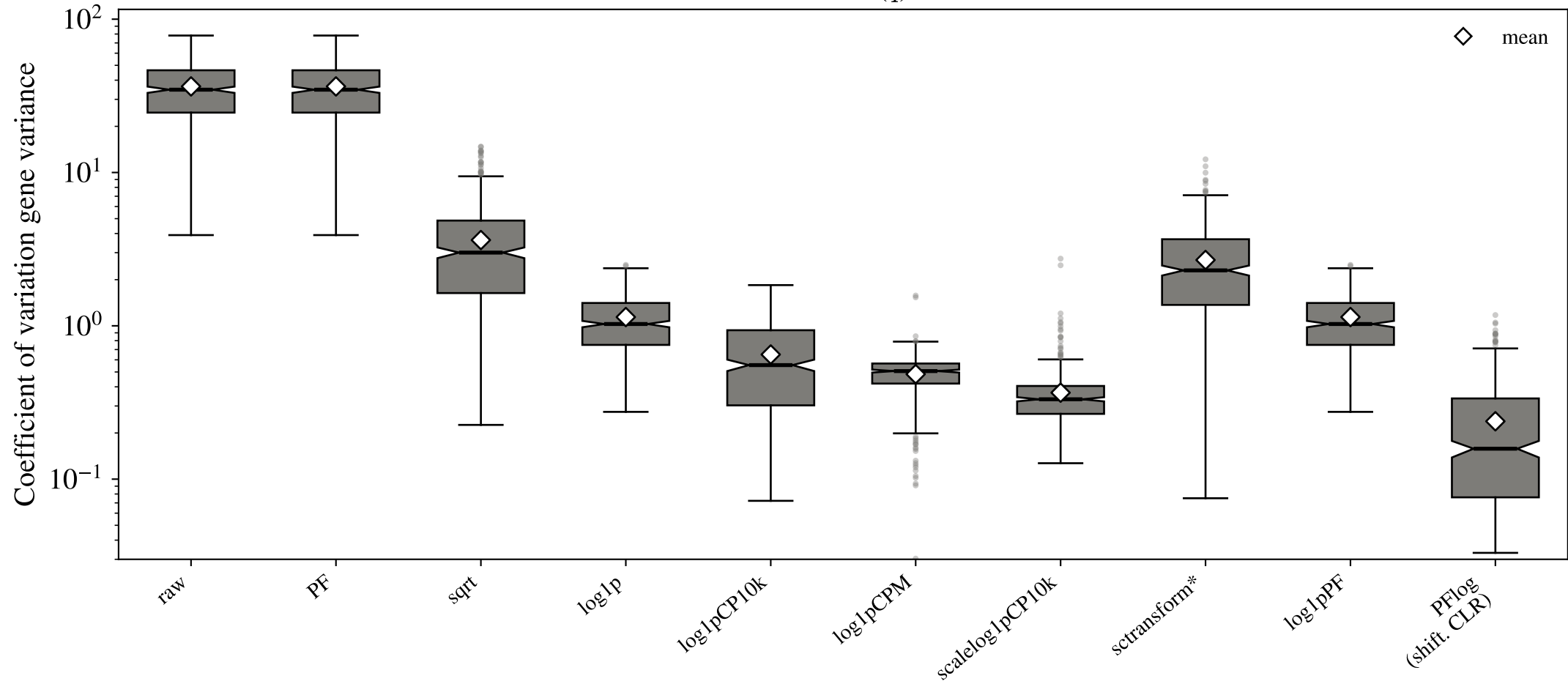
Variance stabilization — CV(q) across 436 datasets
