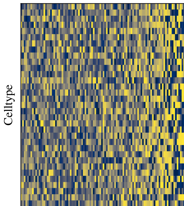
sctransform
