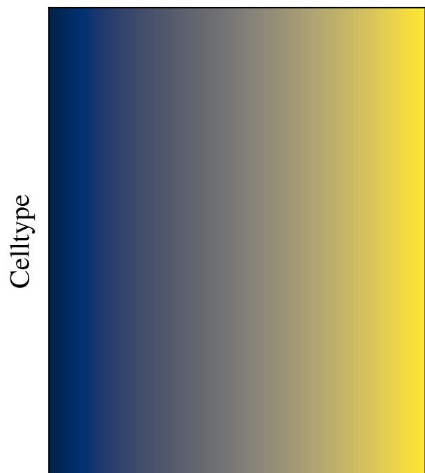
PF
