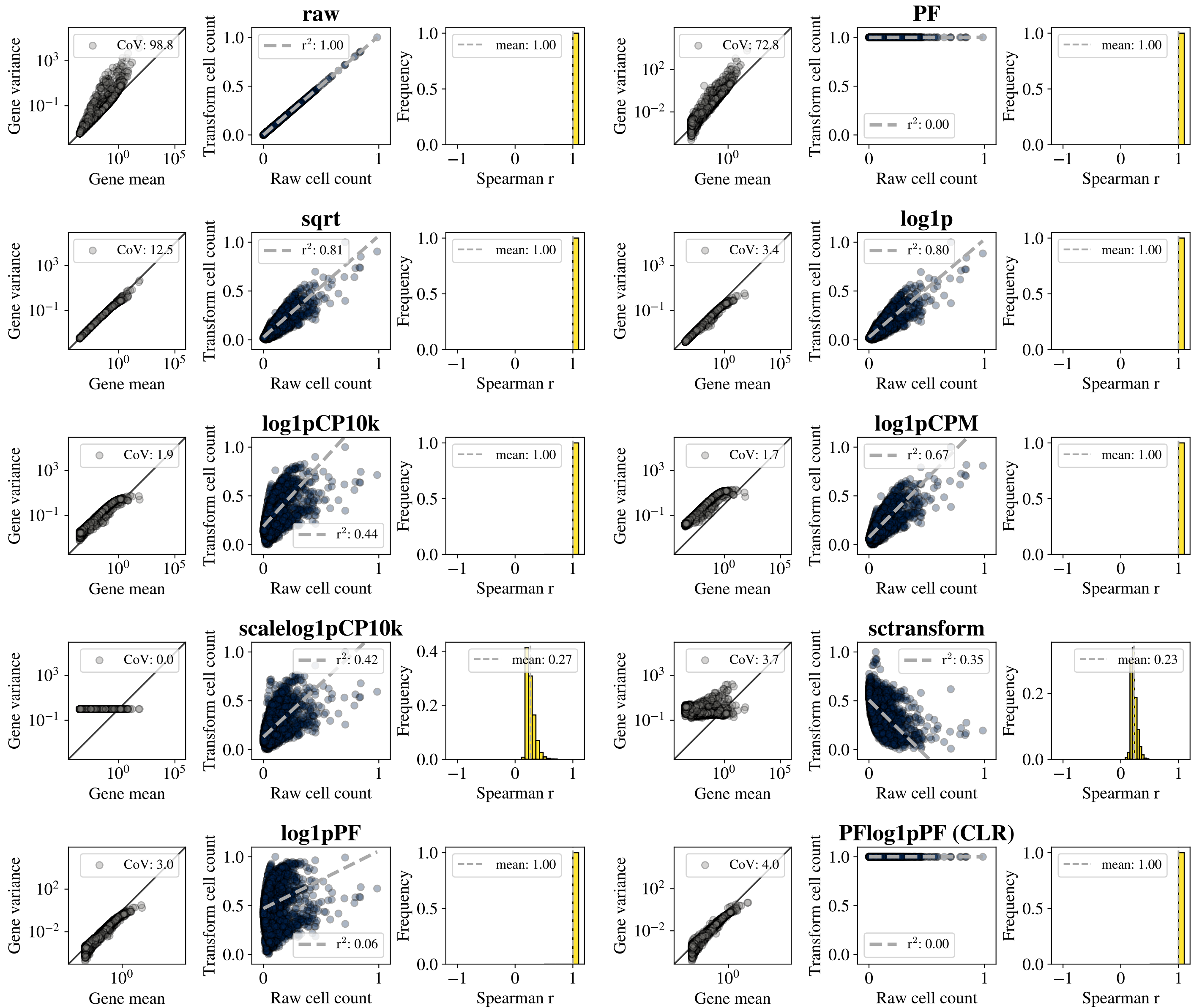
angelidis_2019_subset_genes ( 14,813 \times 16,541 )
