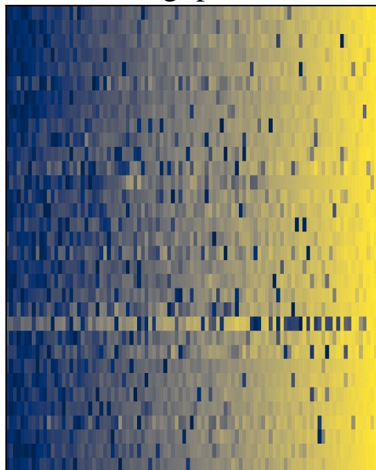
log1pPF
