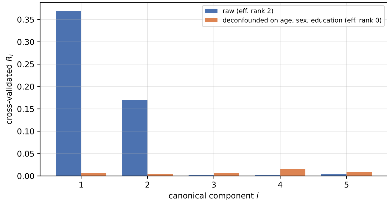
Recoverability with vs. without demographic deconfounding
