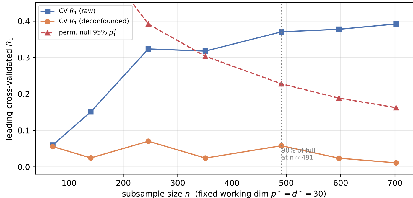
How much data is needed? CV recoverability vs. subsample size
