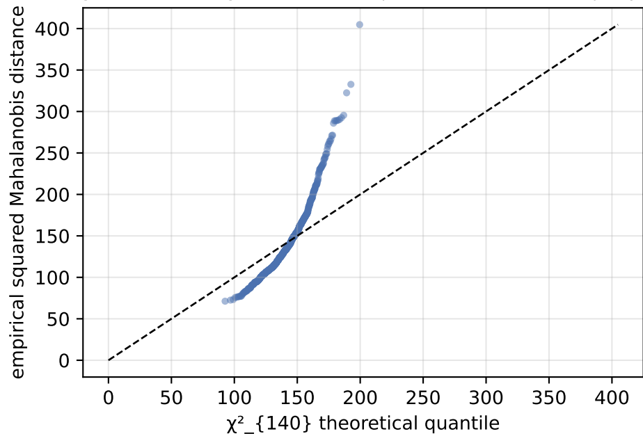
genomics — 140 genomic PCs (raw p=2000 \geq n=702, PCA proxy)
