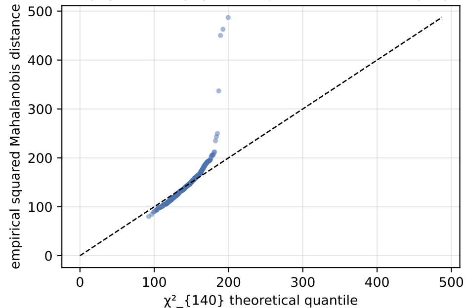
imaging — 140 imaging PCs (raw p=1022 \geq n=702, PCA proxy)
