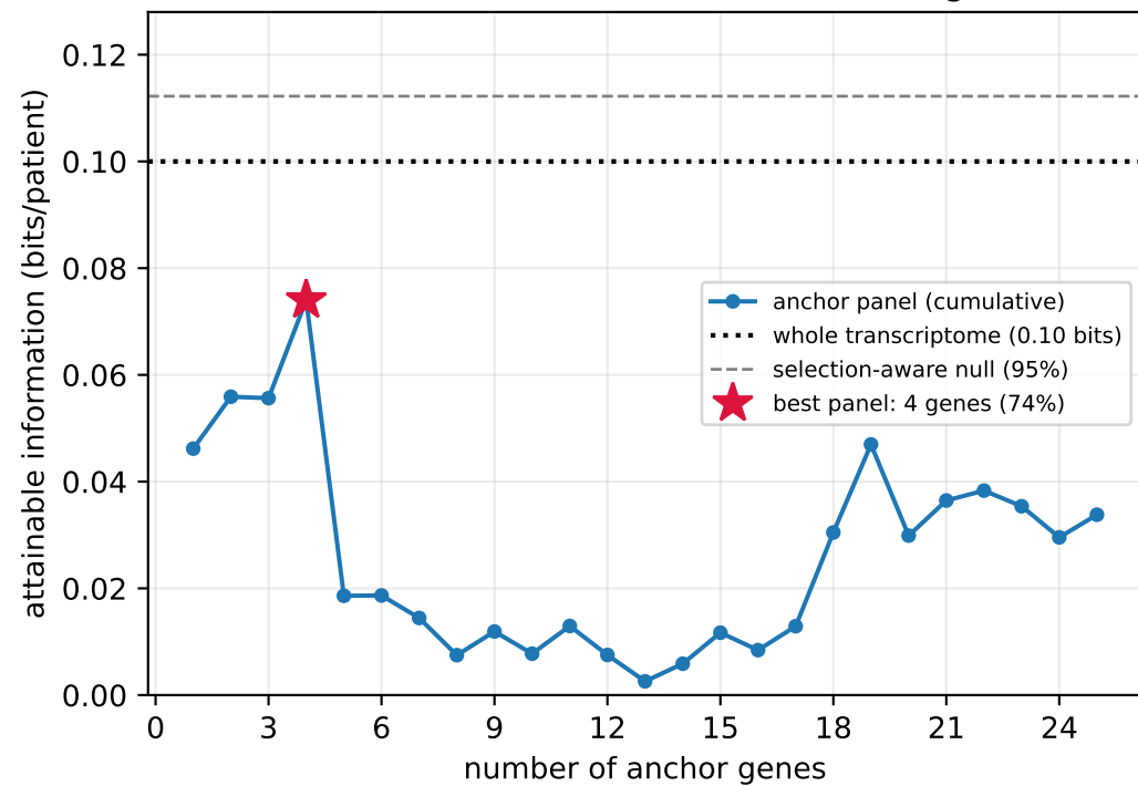
(a) NSCLC: saturation with a handful of genes
